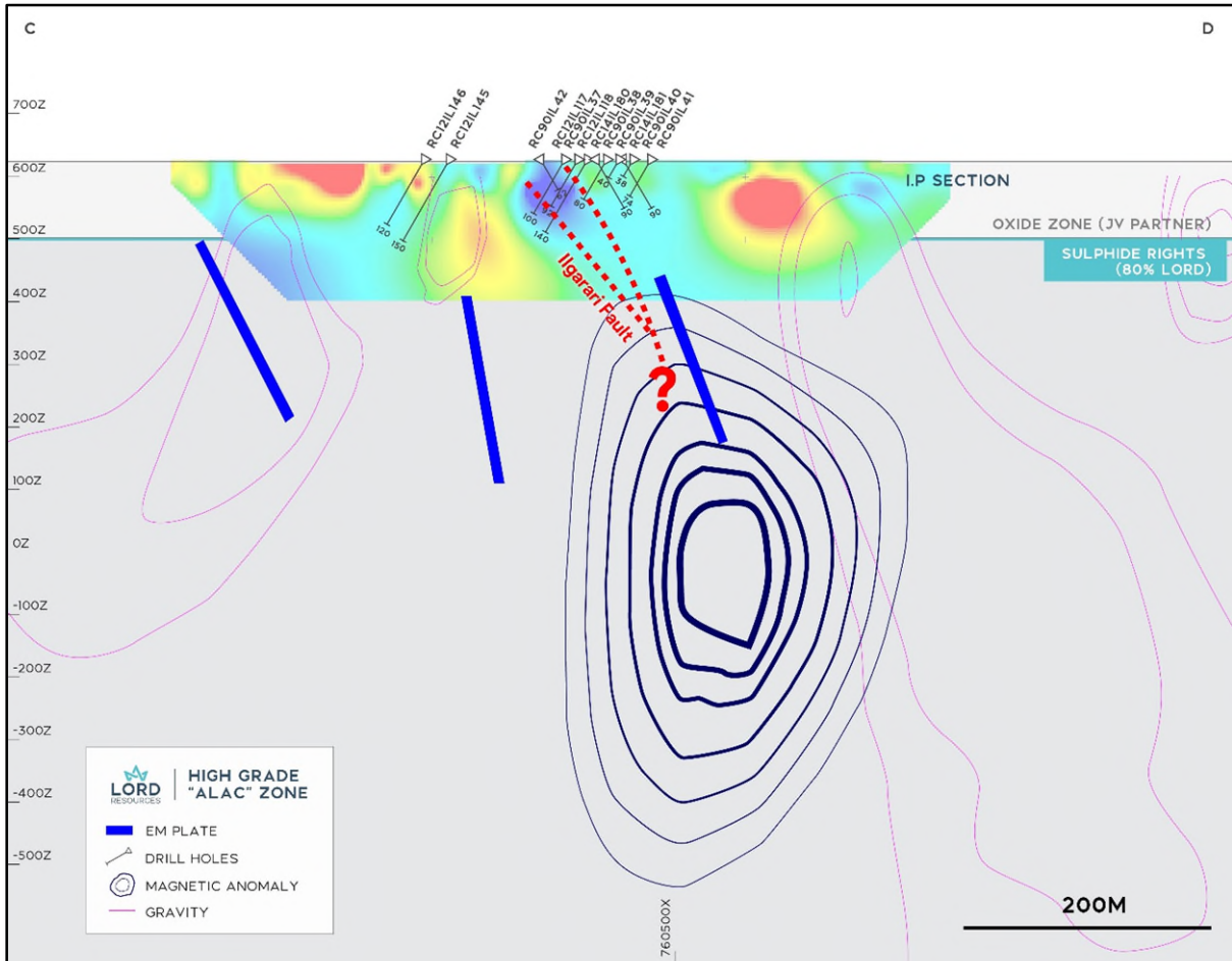
Fig 3: Cross Section of EM plate modelling (blue lines) above the magnetic anomaly (right of image), - "Zone 8" EM plate (centre) and northern EM plates (left). Purple lines represent gravity shells 3 , and dark blue concentric lines TMI
