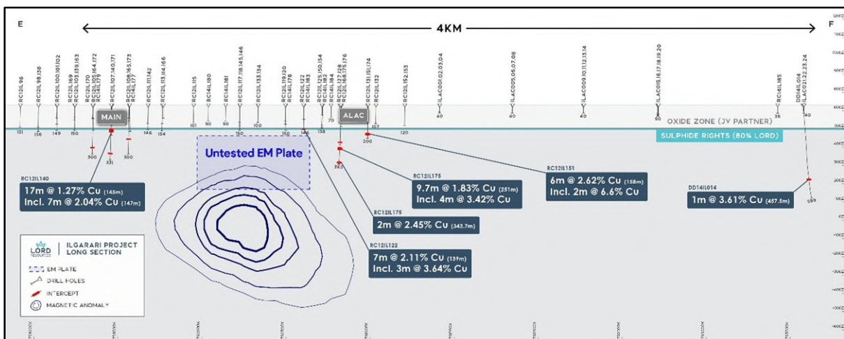
Fig 4: Long Section of EM plate modelling above the magnetic anomaly. Blue lines represent TMI.
