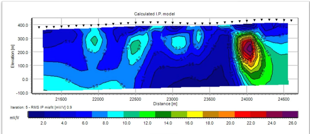
Calculated IP model for L17100 with a peak chargeability centred around 687965mE, 6419540mN (MGA94 Zone 55) and 220m RL.
