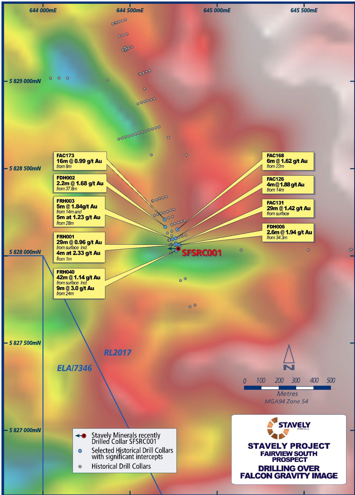
Figure 7. Fairview South gold prospect recent RC drill collar location map overlaid on Falcon™ gravity gradiometer image.
