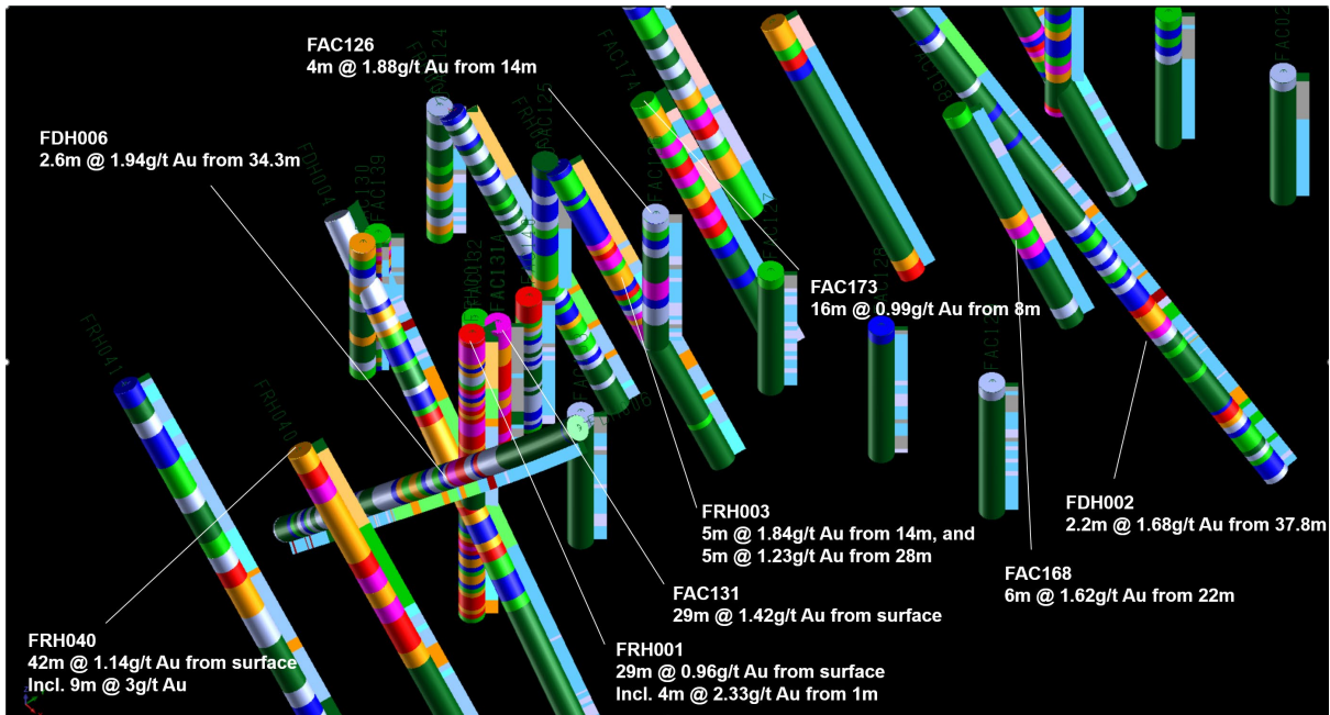
Figure 5. Oblique Surpac™ Fairview South gold prospect scene with gold grades annotated, showing drill holes coloured to gold grade with a lithology colour strip to the right of each hole. Warmer drill trace colours represent higher gold grades. The lithology strip is coloured to geology: blue colours are sediments (sandstone, siltstone and mudstone), orange is undifferentiated weathered material, green are intermediate intrusives, pink are felsic intrusives.
