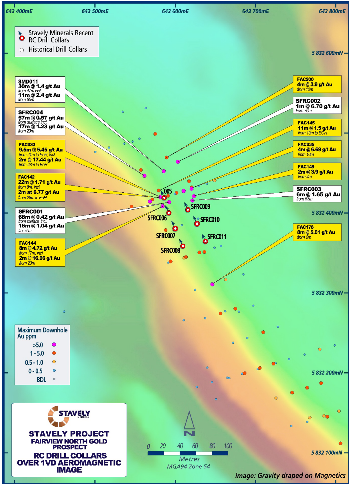
Figure 4. Fairview North gold prospect recent RC drill collar location map.
