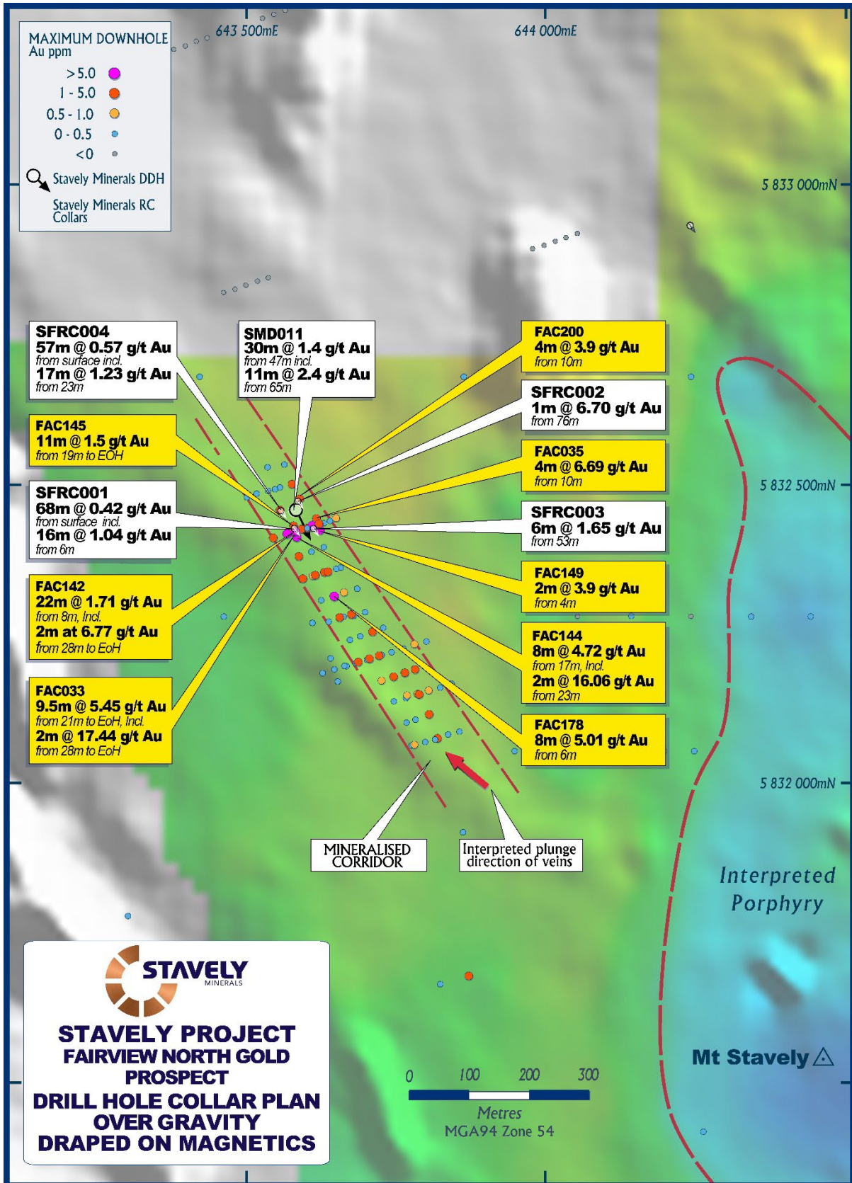
Figure 3. Fairview North gold prospect historic drill-hole location map.
