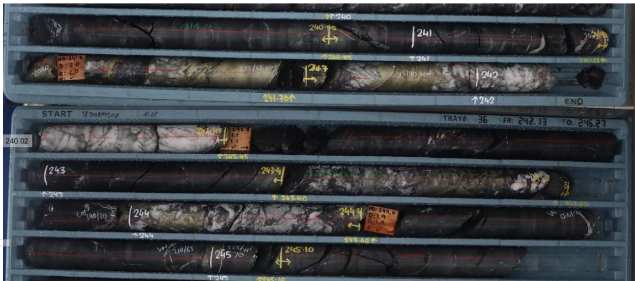
Figure 3: DD24KP1208 intersected 3.08m @ 3.1g/t Au, 4.1% Cu, 30.3g/t Ag from 241.31m. Mineralisation is hosted within a quartz vein with prominent sulphides including 2-20% chalcopyrite, and 1-5% pyrite.
