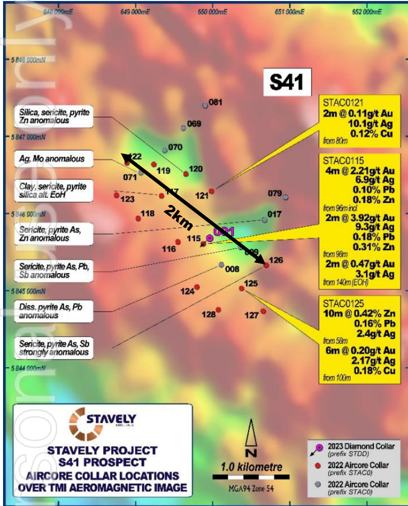
Magnetics
