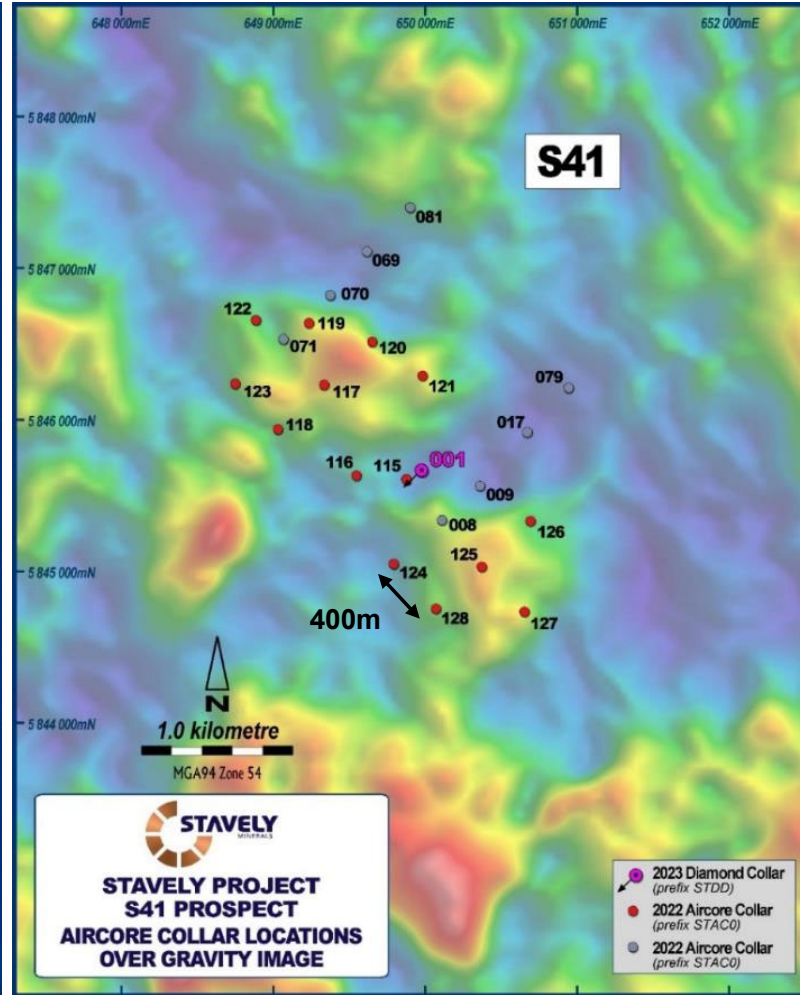
Gravity
