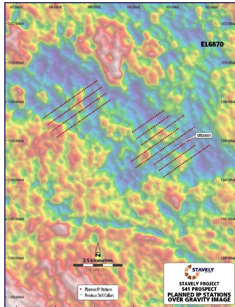
Gravity
