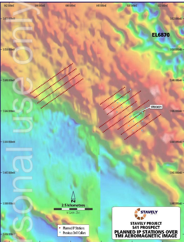
Magnetics
