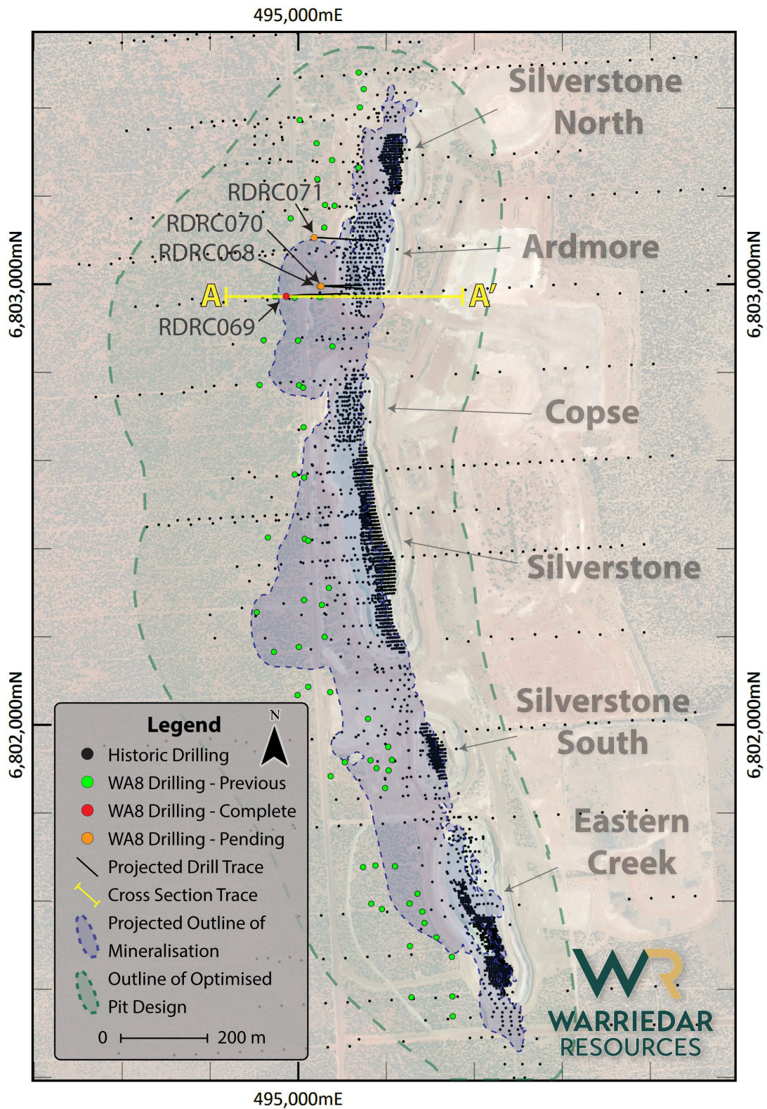
Figure 2: Plan view of Riccardo showing the location of the cross sections in Figures 5 and 6, and the location of drillhole RDR069
