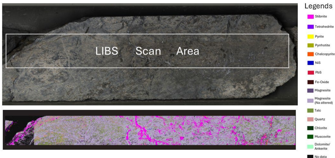
Figure 8: Zoom in EMISSION ECORE LIBS image from core Interval 180.41m to 181.60m (pink is stibnite)
