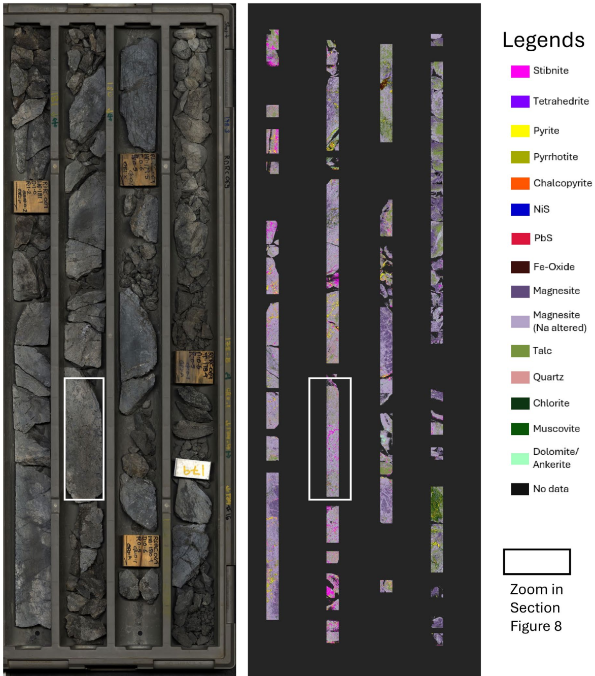
Figure 7: EMISSION ECORE LIBS image from core Interval 178.3m to 181.74m
