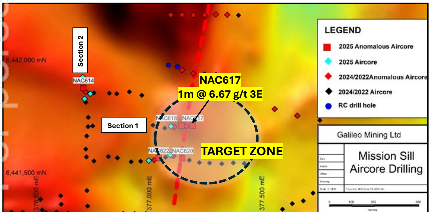
Figure 1 – NAC617 target zone with TMI magnetic background image. See ASX announcement dated 16 th June 2025 for details.
