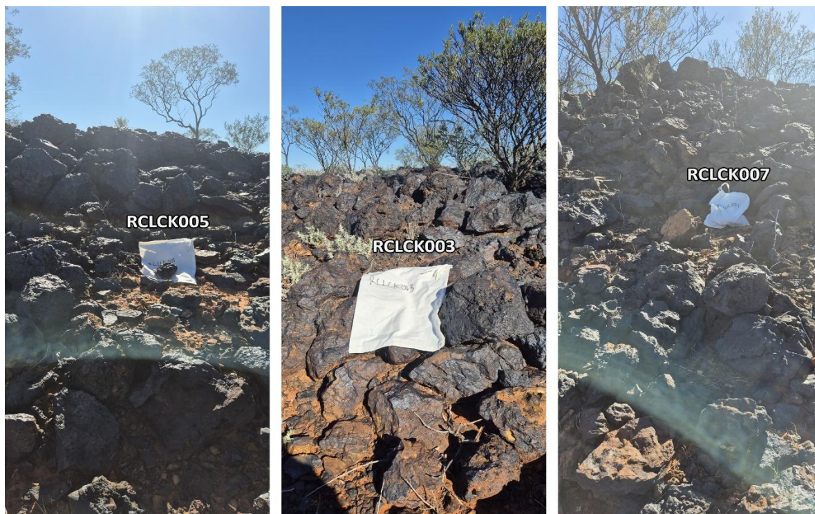
Figure 1. Outcrop photos of sampled massive manganese mineralisation.
