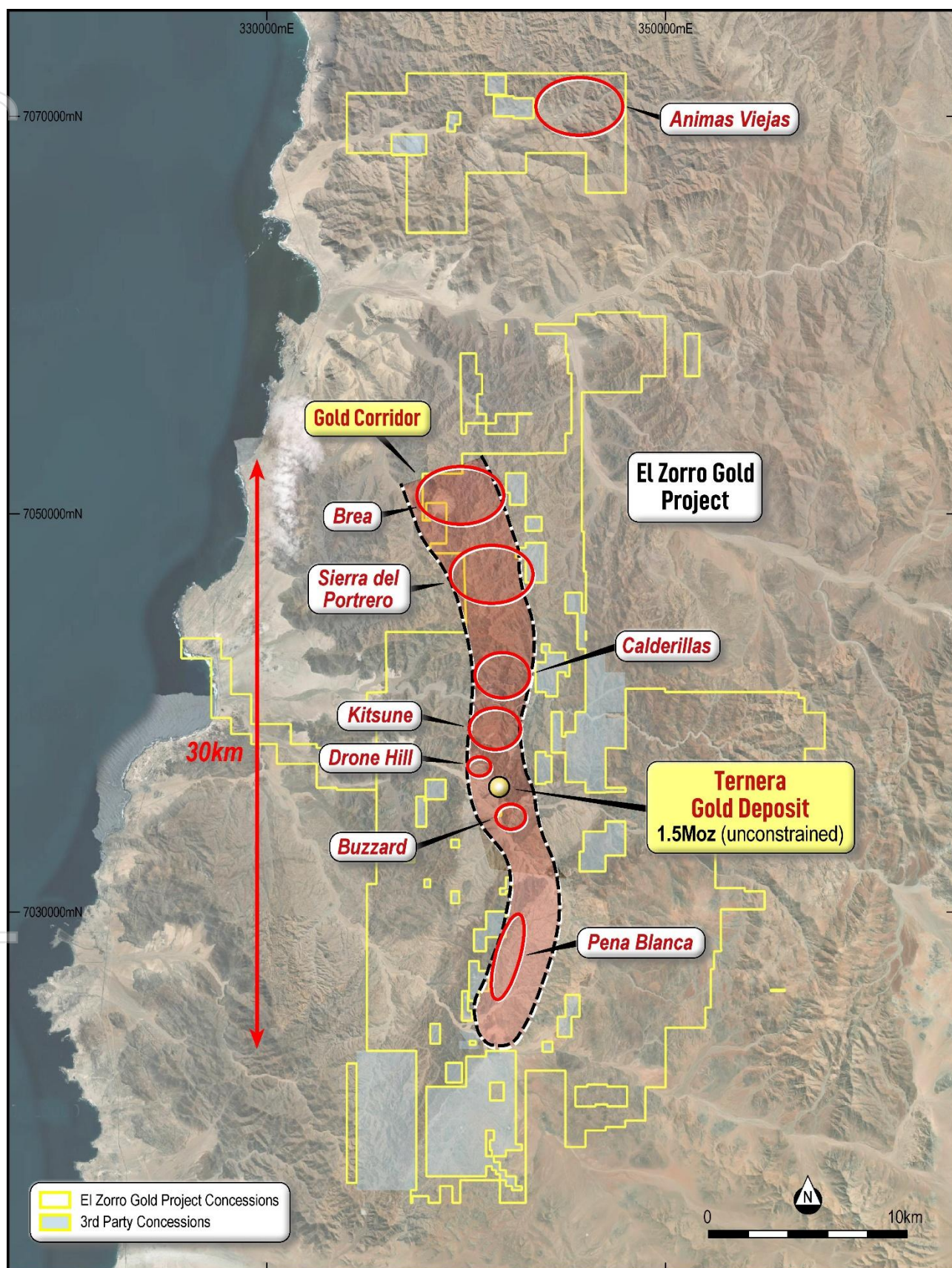
Figure 1: El Zorro Gold Project – District Gold Targets. La Brea is located approximately 15km north of the Terner Gold Deposit Datum PSAD56 19S.
