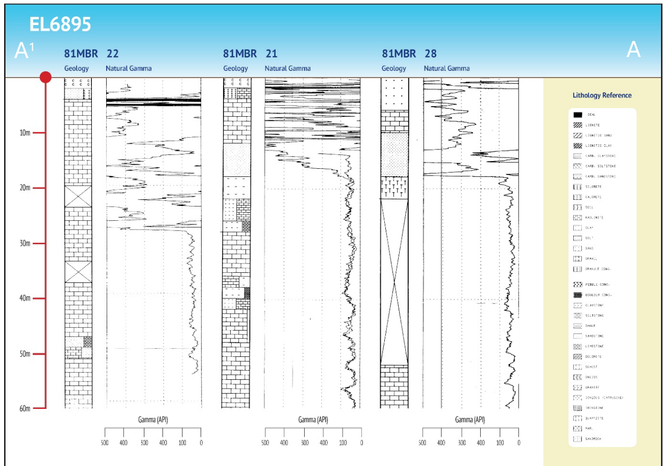
Figure 1: Schematic showing geology and natural gamma traces from 1981 drillholes, extracted from open file envelope ENV3957 pages 364, 365 and 369. Location of drillholes shown in Figure 3 and collar locations included in Appendix 2.
