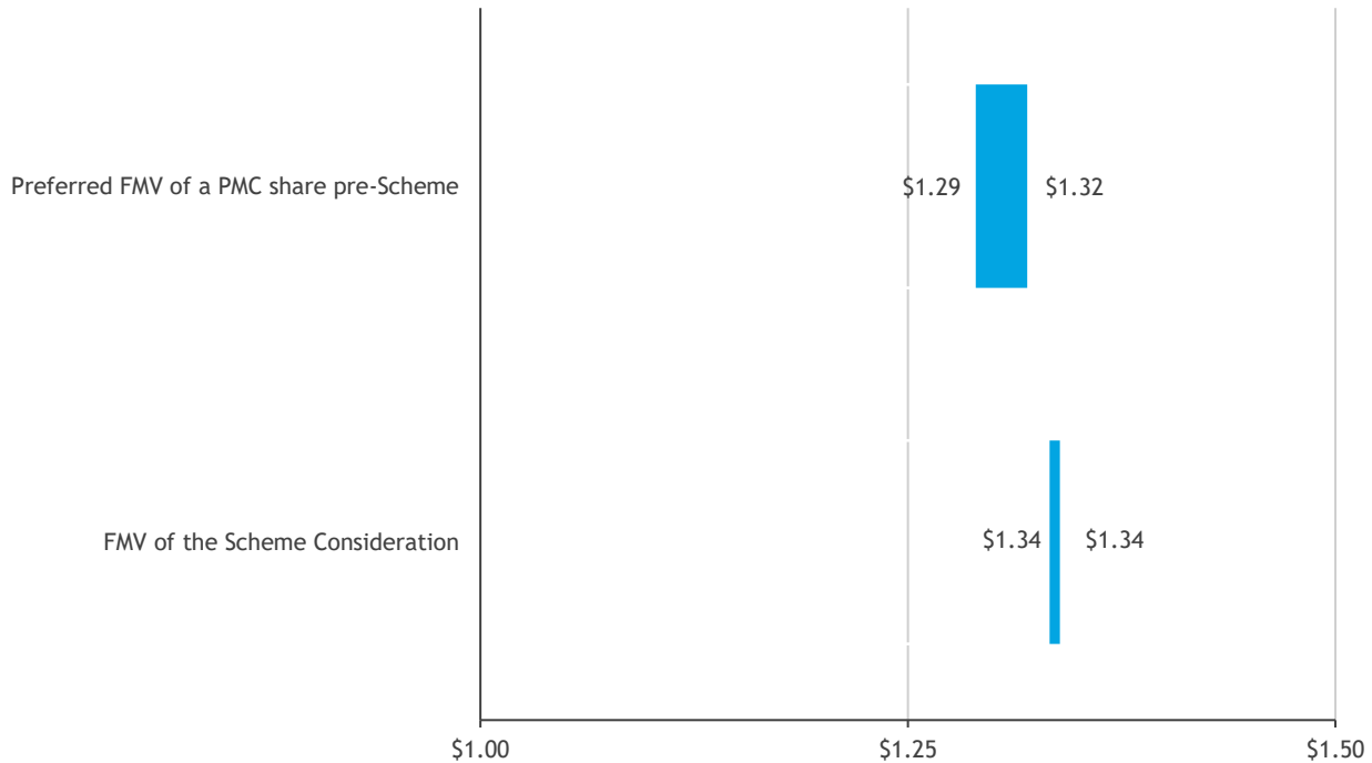
Figure 1: Fairness assessment
