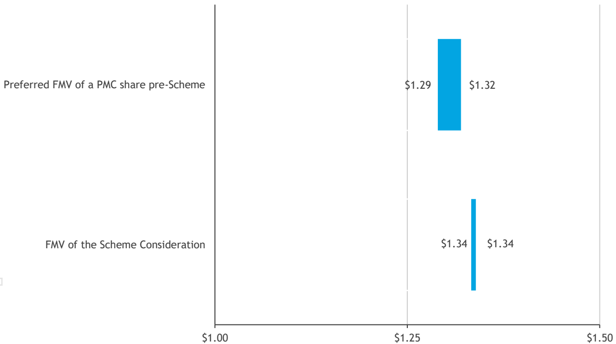
Figure 12: Fairness assessment
