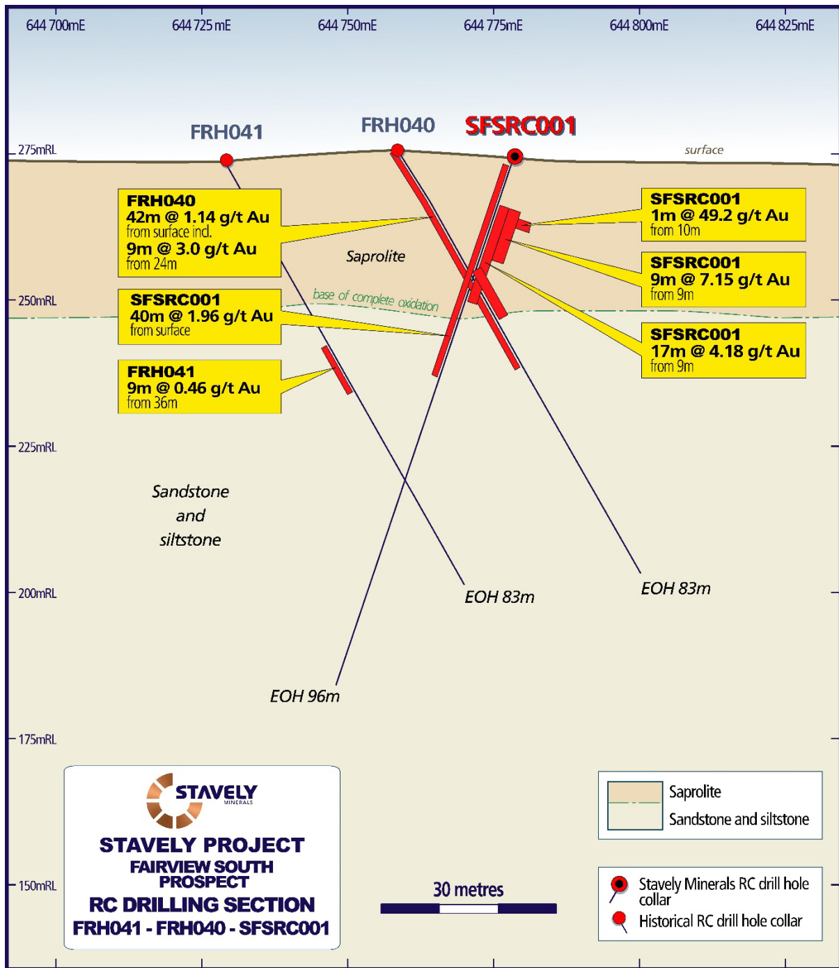
Figure 7. Cross-section of SFSRC001.
