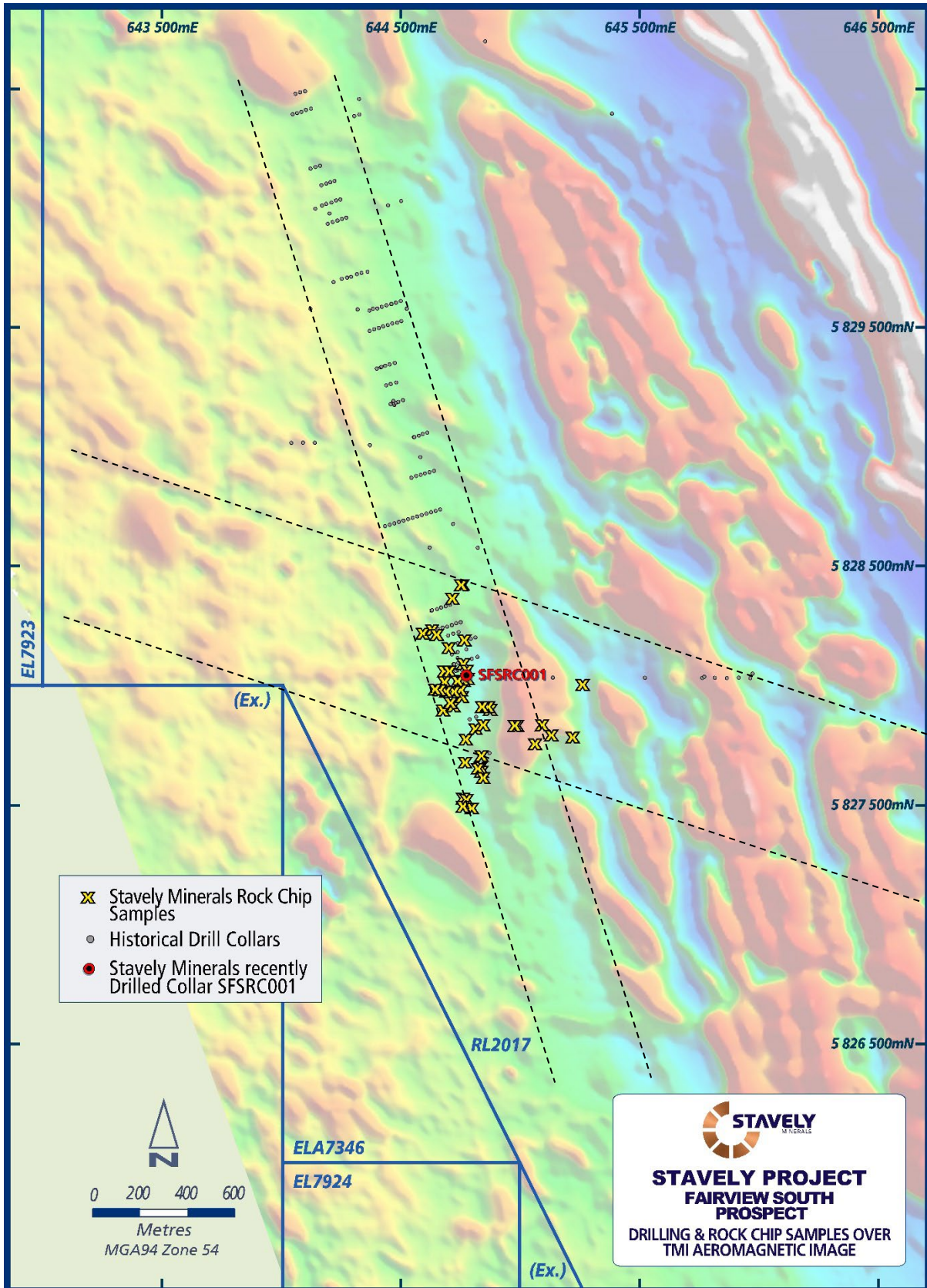
Figure 6. Fairview South gold prospect recent RC drill collar location map and float rock-chip locations overlaid on TMI magnetic image. Note that the Fairview South gold prospect is located at the intersection of the NS Fairview trend and a clear WNW-oriented structural zone.
