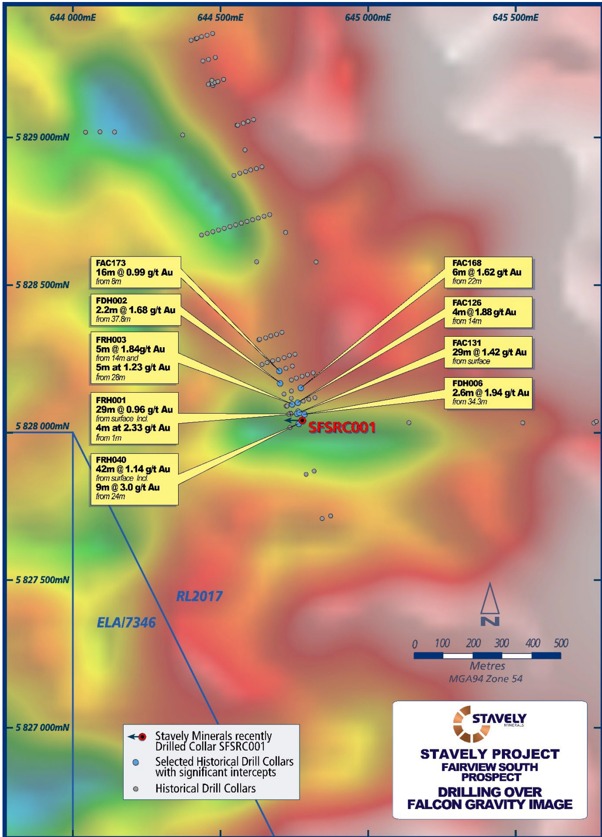
Figure 5. Fairview South gold prospect recent RC drill collar location map overlaid on Falcon™ gravity gradiometer image.
