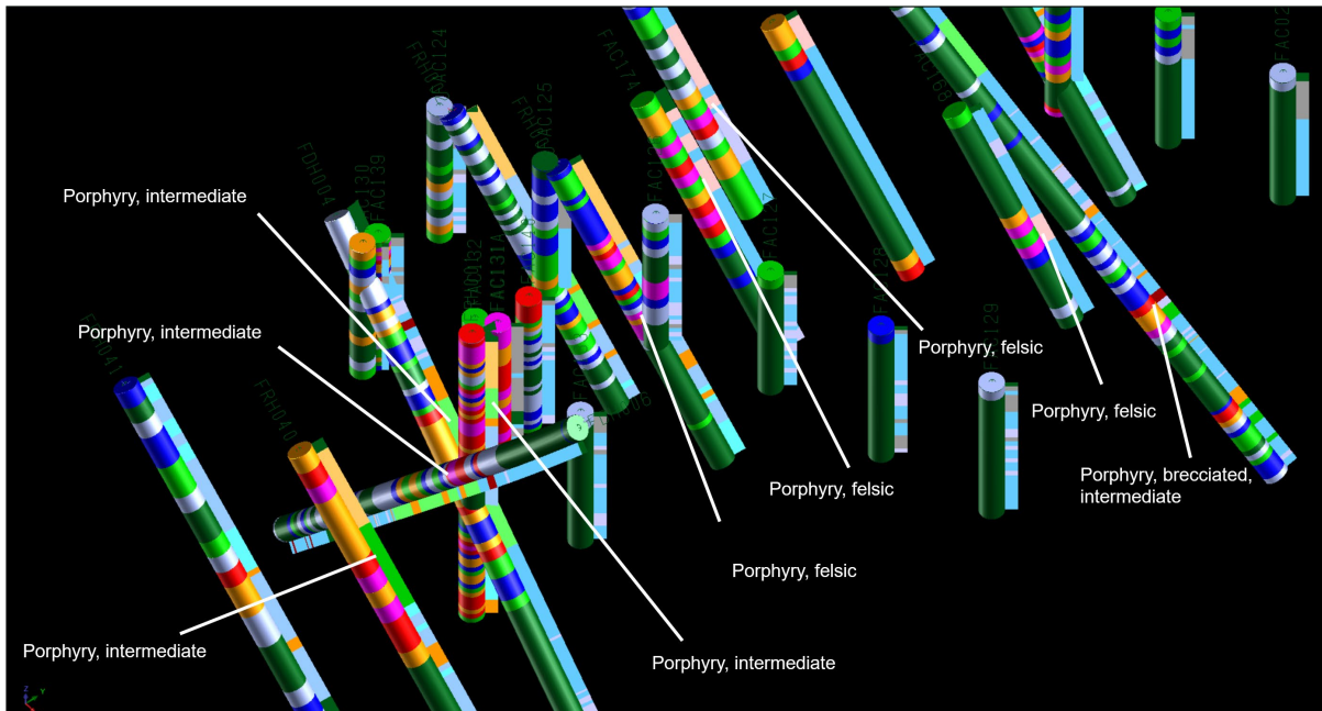
Figure 4. Oblique Surpac™ Fairview South gold prospect scene with showing drill holes coloured to gold grade with a lithology colour strip to the right of each hole. Warmer drill trace colours represent higher gold grades. The lithology strip is coloured to geology: blue colours are sediments (sandstone, siltstone and mudstone), orange is undifferentiated weathered material, green is intermediate intrusives, pink is felsic intrusives. Labels highlight the close relationship between gold mineralisation and intrusive phases.
