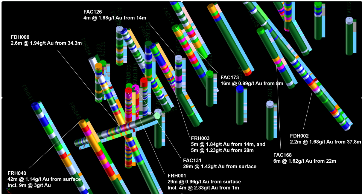
Figure 3. Oblique Surpac™ Fairview South gold prospect scene with gold grades annotated, showing drill holes coloured to gold grade with a lithology colour strip to the right of each hole. Warmer drill trace colours represent higher gold grades. The lithology strip is coloured to geology: blue colours are sediments (sandstone, siltstone and mudstone), orange is undifferentiated weathered material, green are intermediate intrusives, pink are felsic intrusives.
