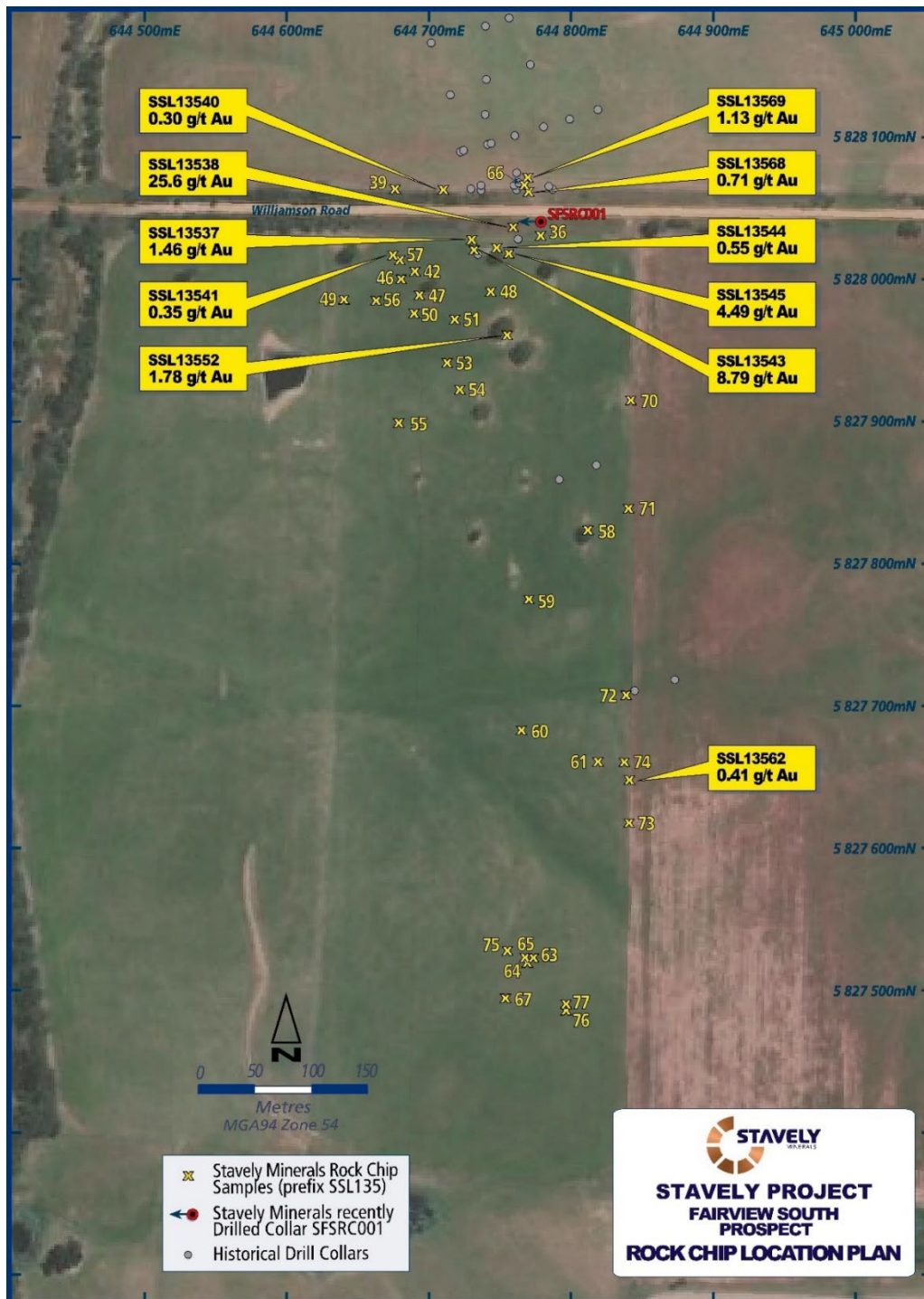
Figure 8. Fairview South gold prospect recent RC drill collar location map and float rock-chip sample locations overlaid on satellite image.
