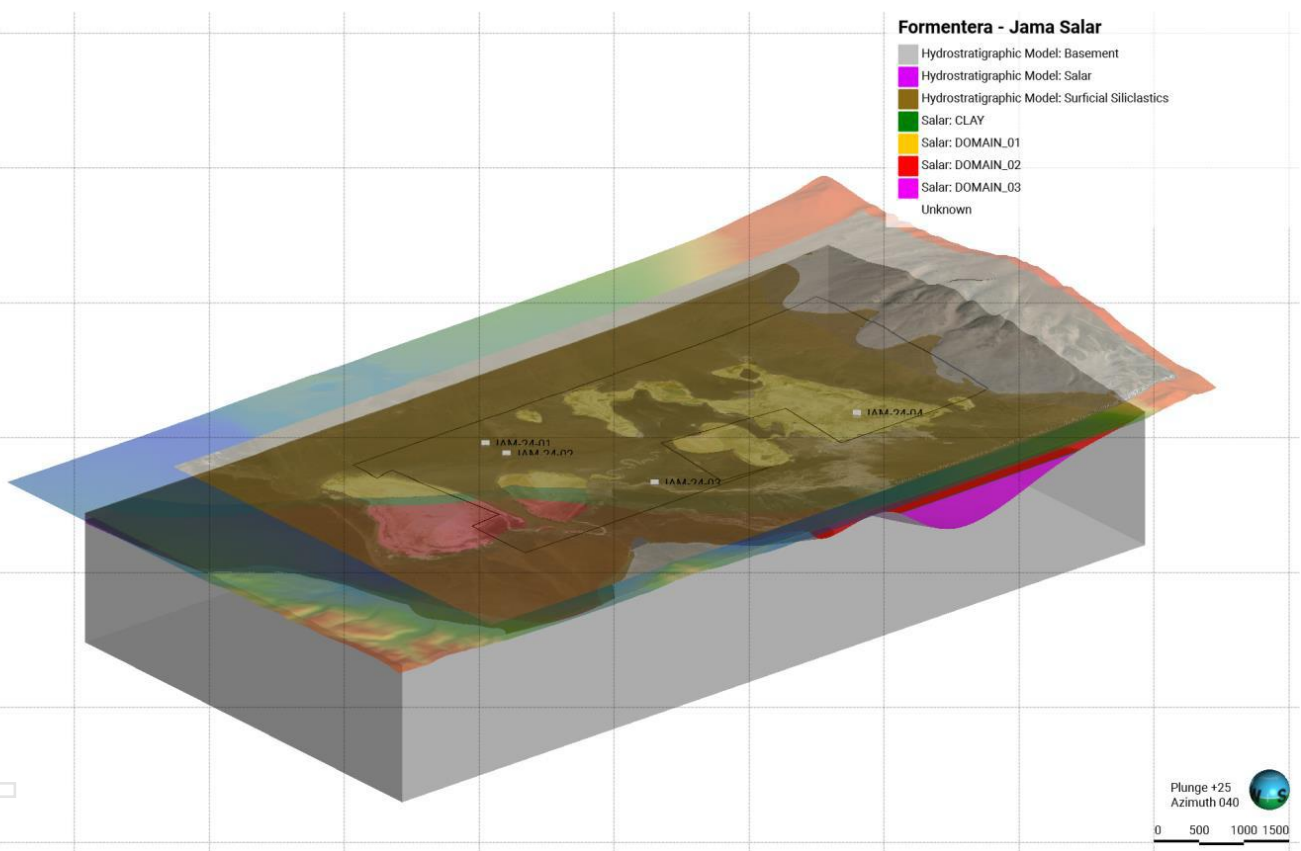
Figure 17. 3D hydrostratigraphic model showing diamond drill hole locations, aerial imagery and topography
