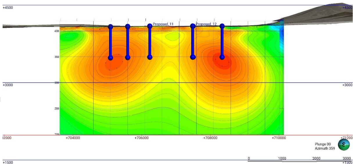
Figure 9. Geophysics line L7410300 in 2D inversion showing drill hole locations in east-west section and high conductivity (orange area) down to 3,000 masl.
