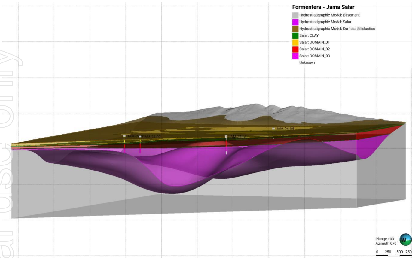
Figure 18. North-west/south-east section through the hydrostratigraphic model, showing modelled continuity.
