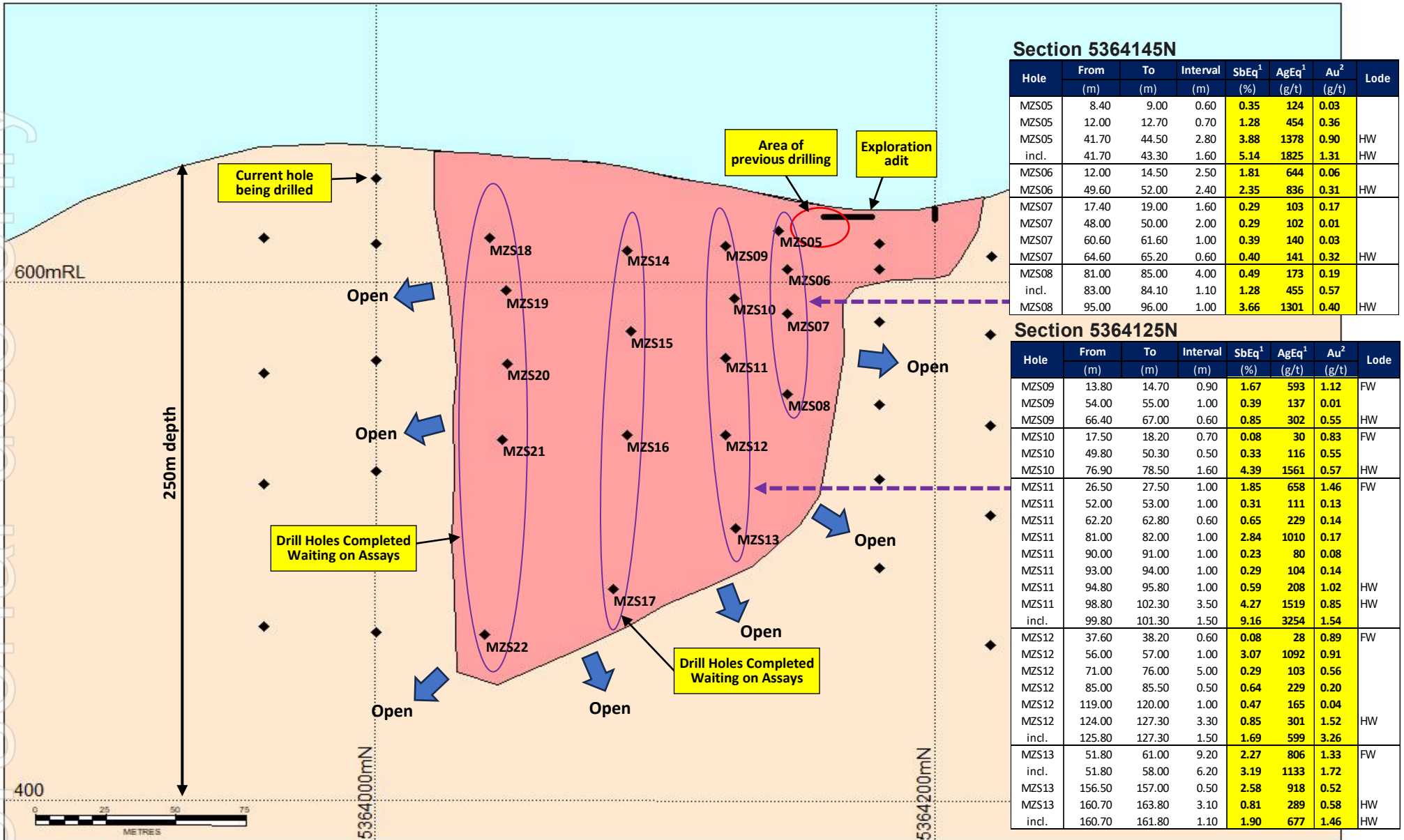
Figure 1. Montezuma Antimony & Silver Lode - hanging wall lode
