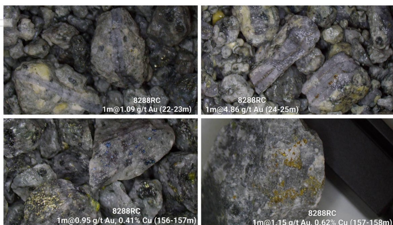
Figure 11: RC chips showing high grade gold in phyllic-altered diorite with disseminated pyrite-chalcopyrite ± bornite and B-type veins.
