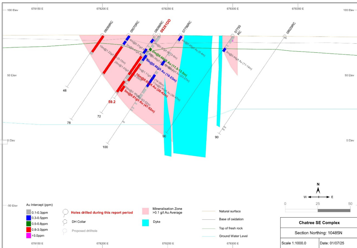
Figure 7: Significant gold intercepts 13 in section 10485N 14 , Western Zone of Chatree South-East Complex.
