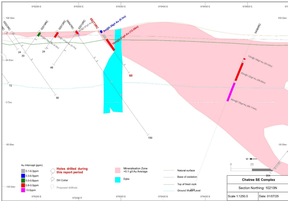
Figure 6: Significant gold intercepts 11 in section 10210N 12 , Western Zone of Chatree South-East Complex.
