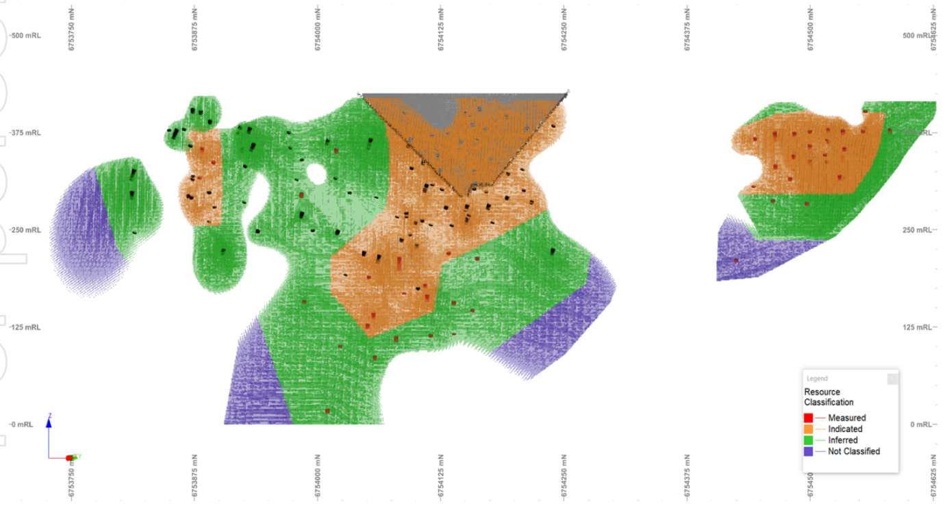
Figure 3, Long section through the extended Swiftsure and proposed Pit 9 with new Tiptoe lodes on the right. Representing Resource categories for July 2025 MRE. (Orange - Indicated, Green - Inferred and Blue - unclassified)
