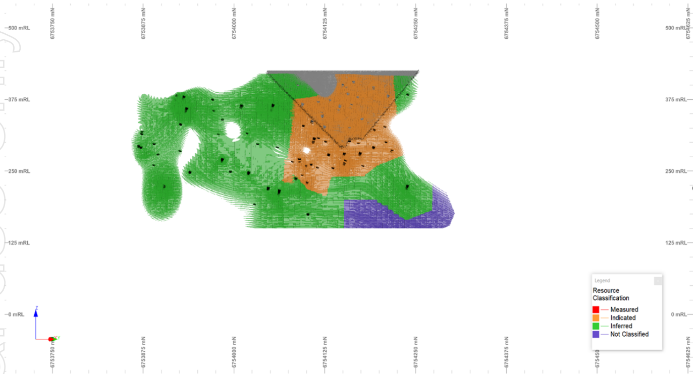
Figure 2, Long section through the Swiftsure lodes and proposed Pit 9 representing Resource categories for June 2024 MRE. (Orange - Indicated, Green - Inferred and Blue - unclassified)
