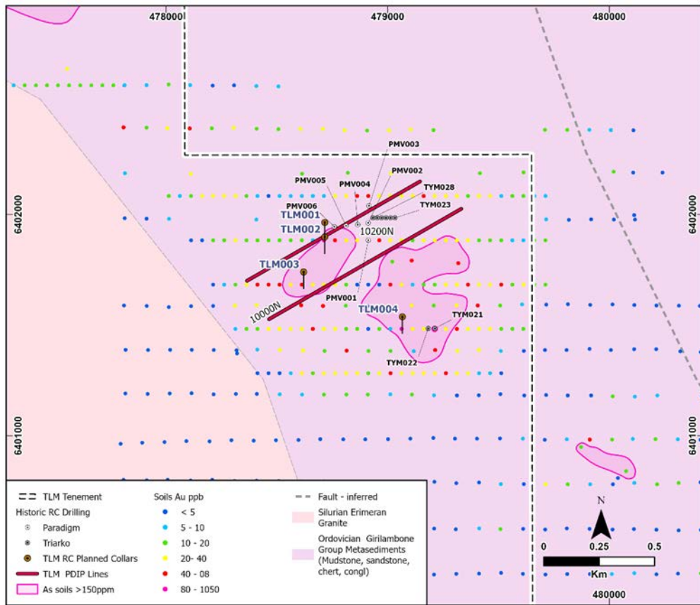
Figure 3. Sheepyard target within the Walkers Hill geochemical gold trend. Coherent gold and arsenic-in-soil anomaly with location of TLM PDIP lines, historic drilling and planned TLM RC holes.
