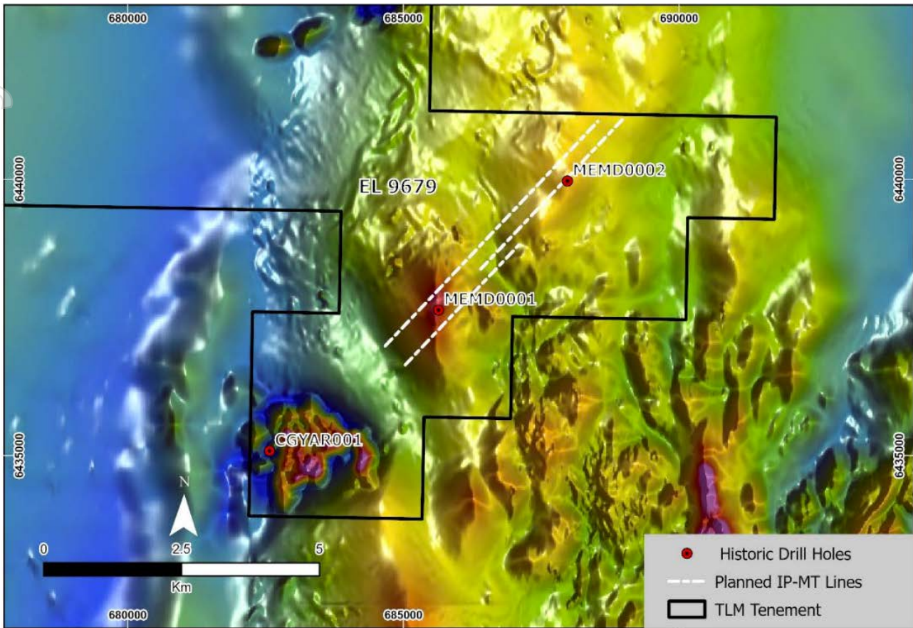
Figure 4: Yarindury Project area on magnetic image (RTP). Planned Ground geophysical IP (Induced Polarisation) and MT (Magnetotelluric) Survey line locations are illustrated.
