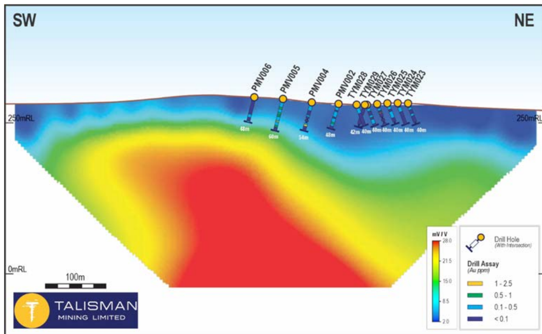
Figure 4: Sheepyard target PDIP section 10200 within the Walkers Hill geochemical gold trend. The large IP chargeability anomaly sits below a significant, coherent gold and arsenic-in-soil anomaly and below intercepts of 40m at 0.46g/t Au from 3m and 12m at 0.38g/t from surface in shallow RC drilling. Talisman's initial RC drilling program will test the IP anomaly at depths up to 200m below surface. (For drill hole locations, see Figure 3).
