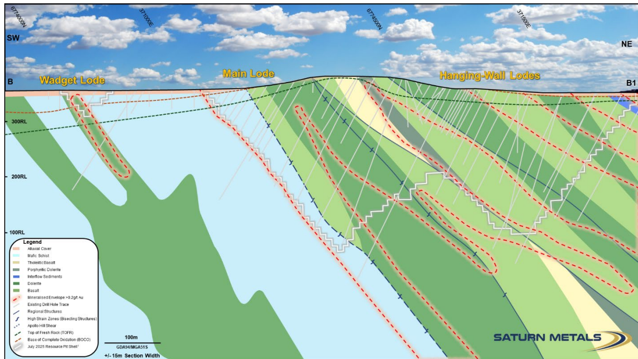
Figure 8 – Apollo Hill Geological Interpretation in southwest-northeast cross section (+/- 15m) B-B 1 location illustrated in plan view on Figure 7; completed and planned drill holes (current program) also illustrated.
