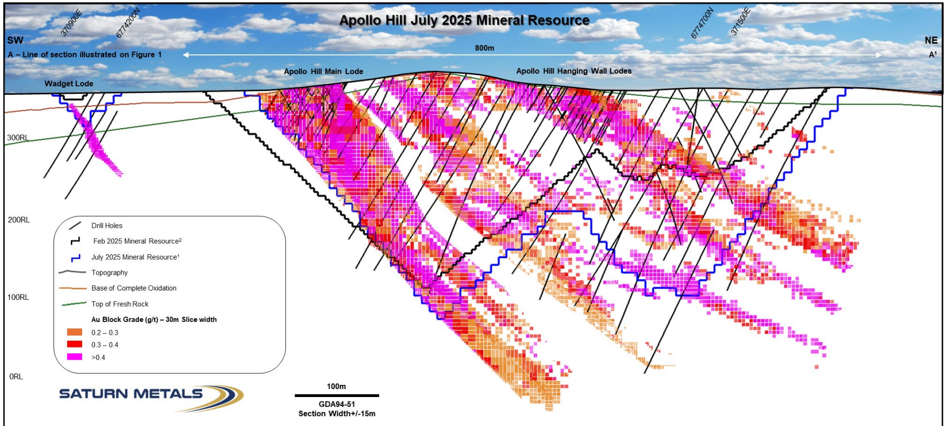
Figure 2 – Oblique block model cross-section (South West – North East, A-A' on Figure 1 3D diagram) ± 15 m showing gold grade and block locations.
