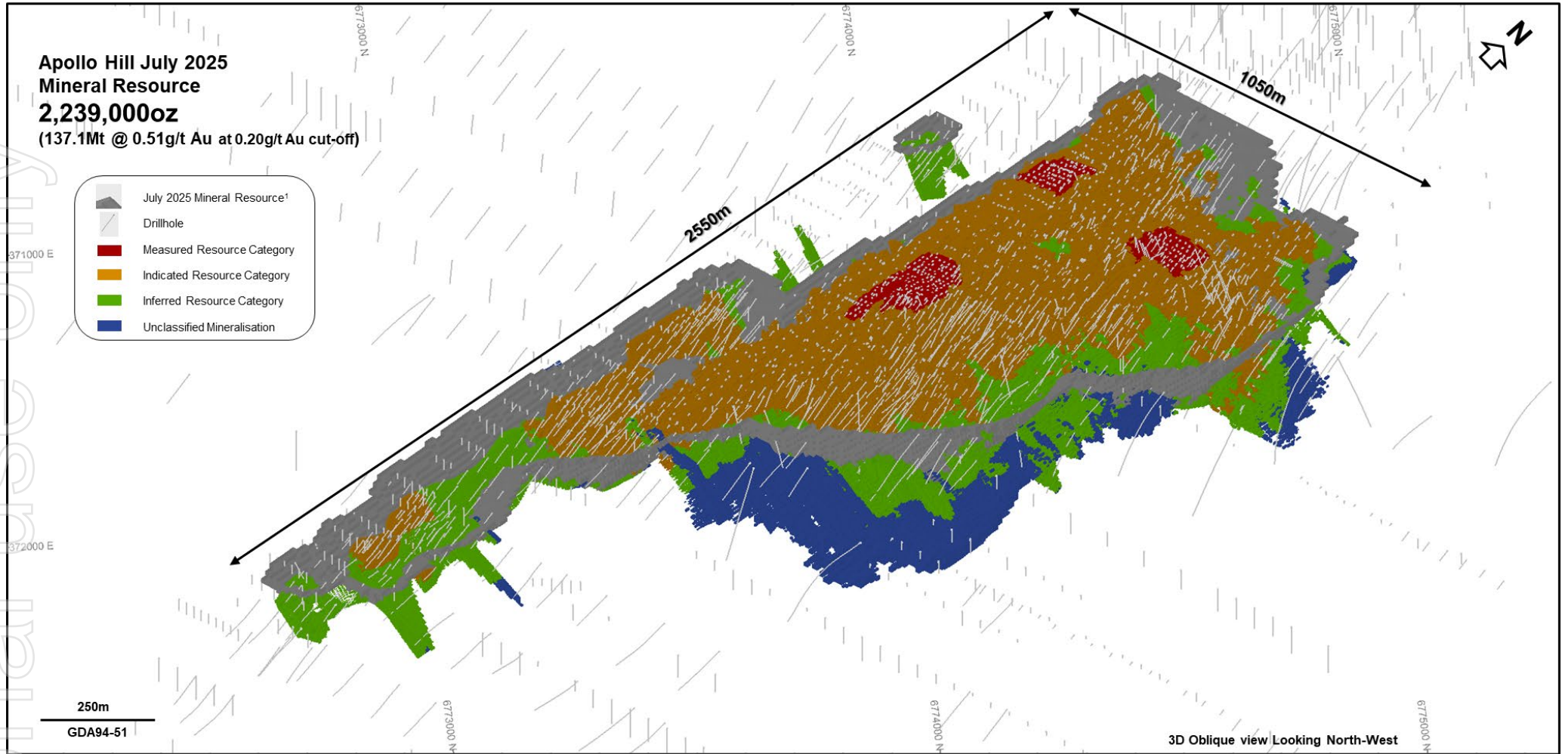
Figure 3 – Measured, Indicated, Inferred Mineral Resource and unclassified mineralization relative to the nominal constraining open pit shell. Blocks illustrated are >0.20 g/t Au (cut-off grade). Material outside of the nominal pit shell and material left as unclassified is not reported.
