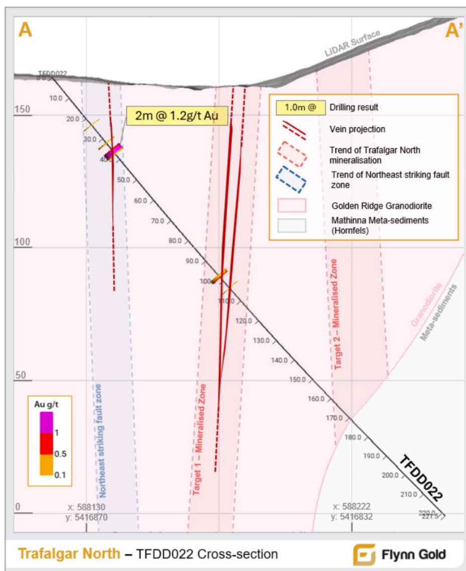
Figure 7 – TFDD022 Cross-Section.
