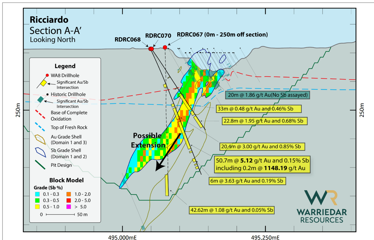
Figure 7: Cross section A-A' – see Figure 3 for location; with Sb Block Model as background. The interval of 0.2m @ 1148.19g/t from RDR068 was reported on 18 June, and the full assays for that hole are reported in this release.
