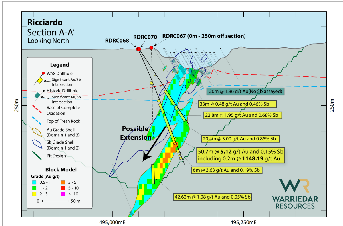
Figure 6: Cross section A-A' – see Figure 3 for location; with Au Block Model as background. The interval of 0.2m @ 1148.19g/t from RDR068 was reported on 18 June, and the full assays for that hole are reported in this release.
