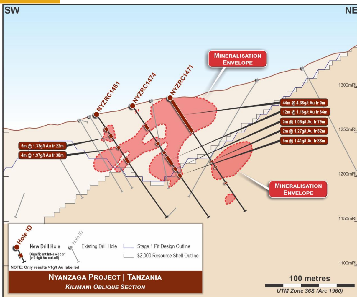
Figure 8: Kilimani Deposit – Oblique cross section looking northeast showing selected new intercepts and historical drill traces
