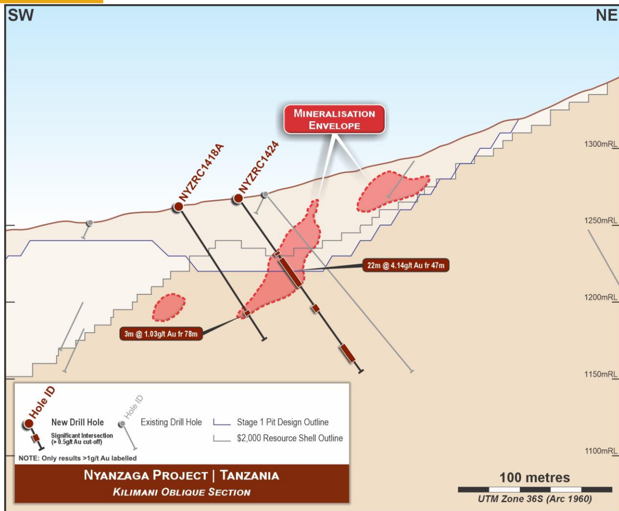
Figure 9: Kilimani Deposit – Oblique cross section looking northeast showing selected new intercepts and historical drill traces
