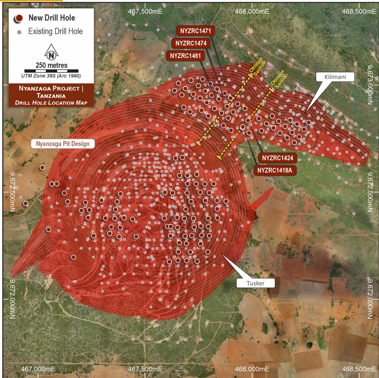
Figure 3: Nyanzaga Gold Project drill plan showing drill collars forming this release with Ore Reserve pit design
