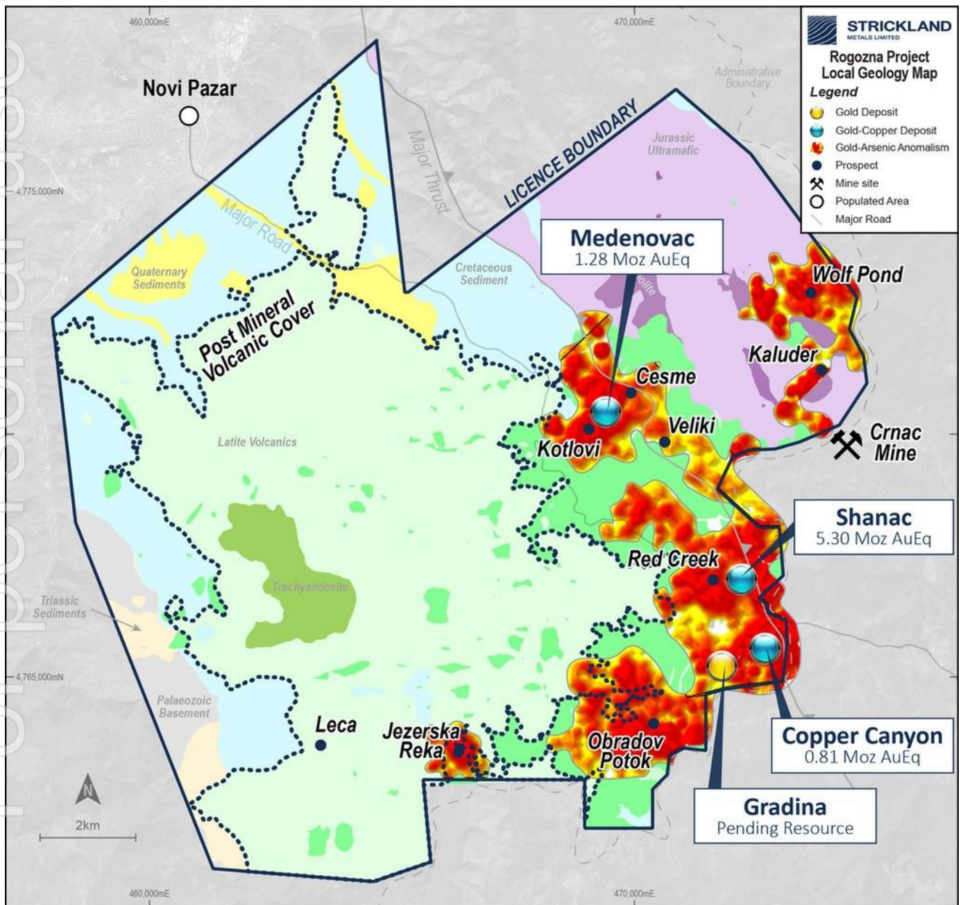
Figure 1. Rogozna Project – Geology, Deposits and Prospects.
