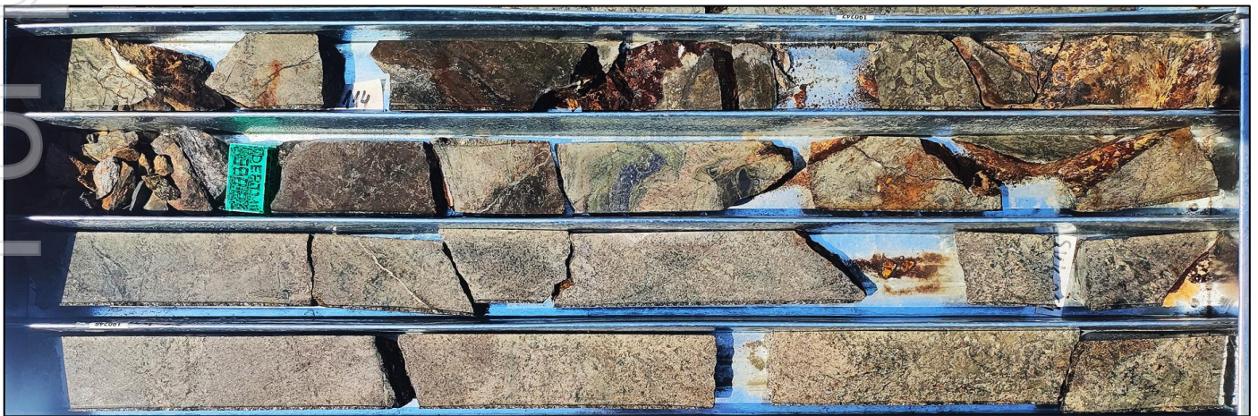
Figure 5. Core photograph from 387.0m to 391.0m in ZRSD25190 showing strong pyrrhotite alteration - 14.8g/t Au.
