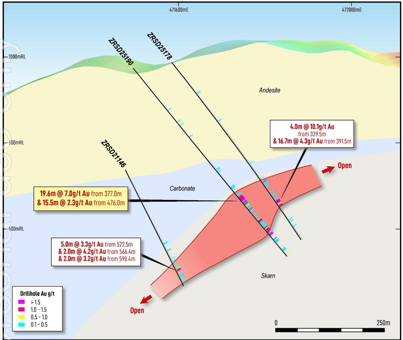
Figure 3. Gradina cross-section view along A-B, showing results for ZRSD25190 in relation to previously reported drill intercepts.
