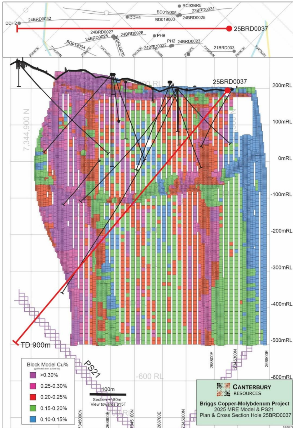
Figure 3 Plan & cross-section of Briggs displaying the 900m deep hole (25BRD0037), historical drilling (projected ±80m) plus the MRE block model
