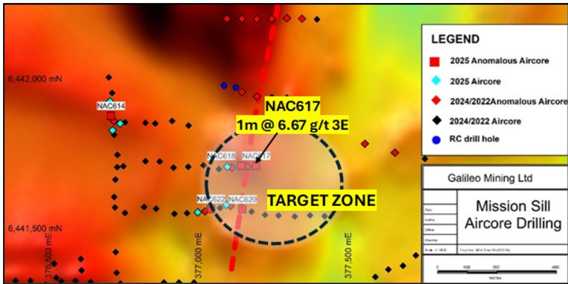
Figure 3 – Central Mission Sill aircore drilling target zones. TMI magnetic background image. See ASX announcement dated 16 th June 2025 for details.
