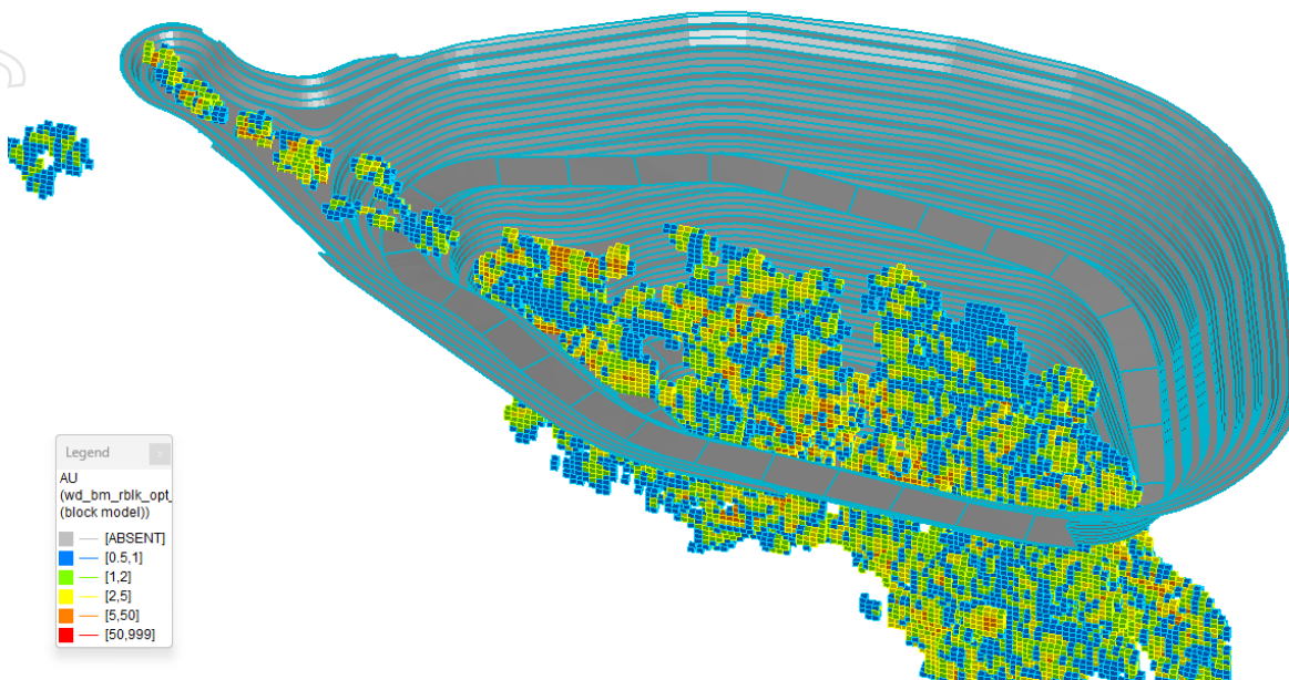
Figure 16: Isometric view of final (stage 3) pit design with block model grades
