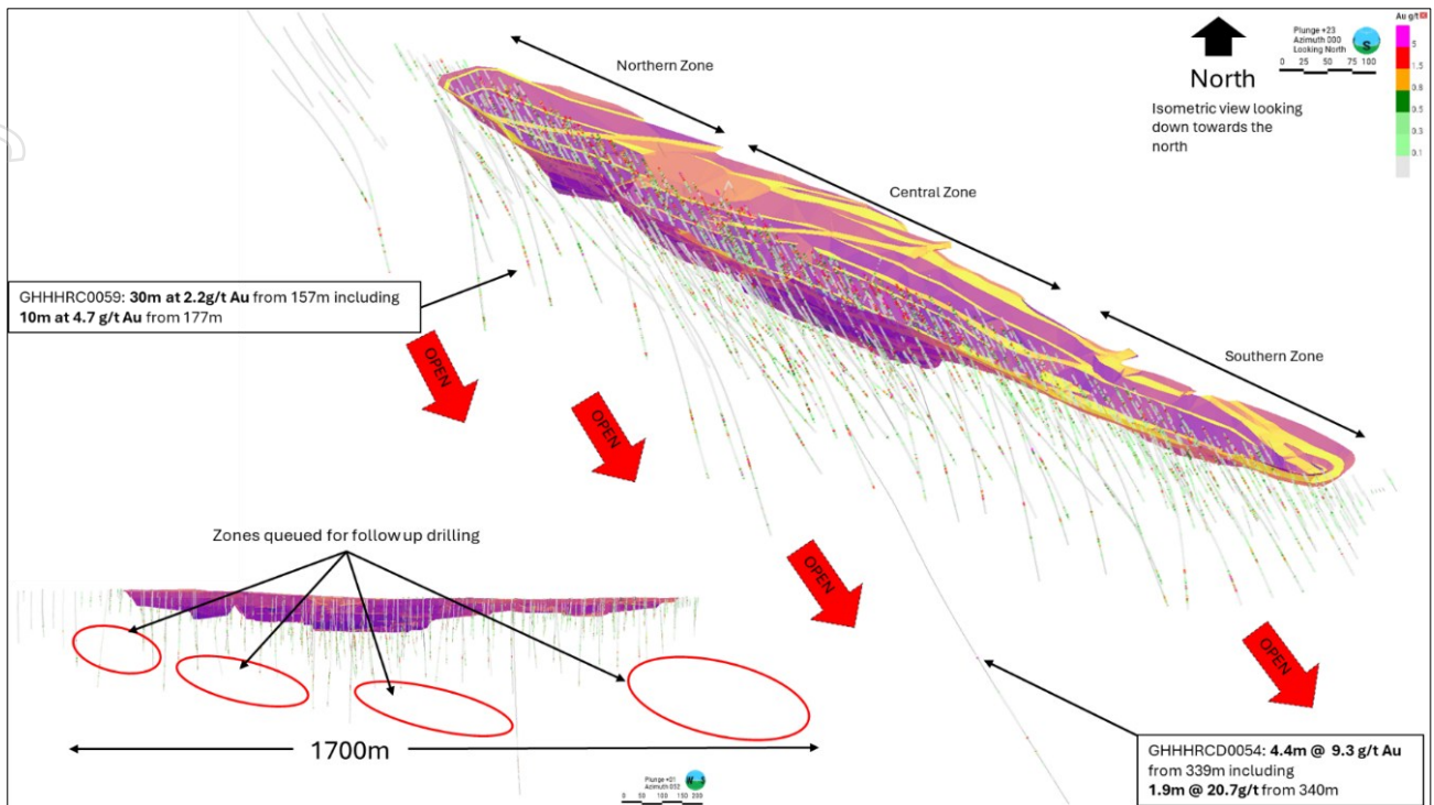
Figure 1: Isometric view (& long section) of projected plunge of current high-grade intersections indicating areas for follow up drilling.
