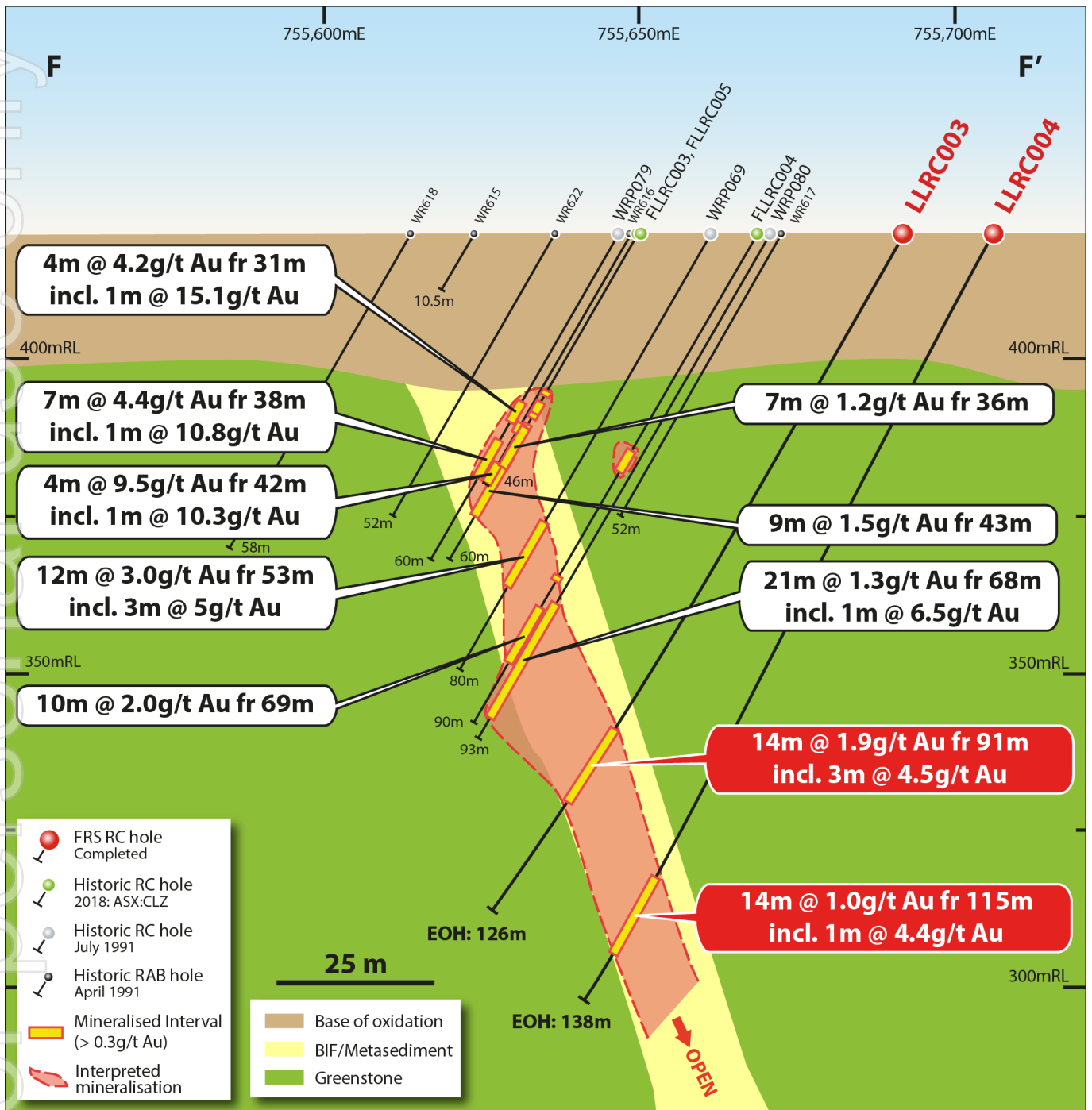
Figure 9. Cross section (F-F'), looking north ~15m along strike, showing Au mineralisation of historic and FRS drilling. Drilling intercept widths are down-hole widths and not true widths. Intercepts are based on a cut-off grade of 0.3g/t Au, allowing for internal dilution by two “waste” or sub-grade (<0.3g/t Au) samples. FRS holes (red caption) were completed in 2021.
