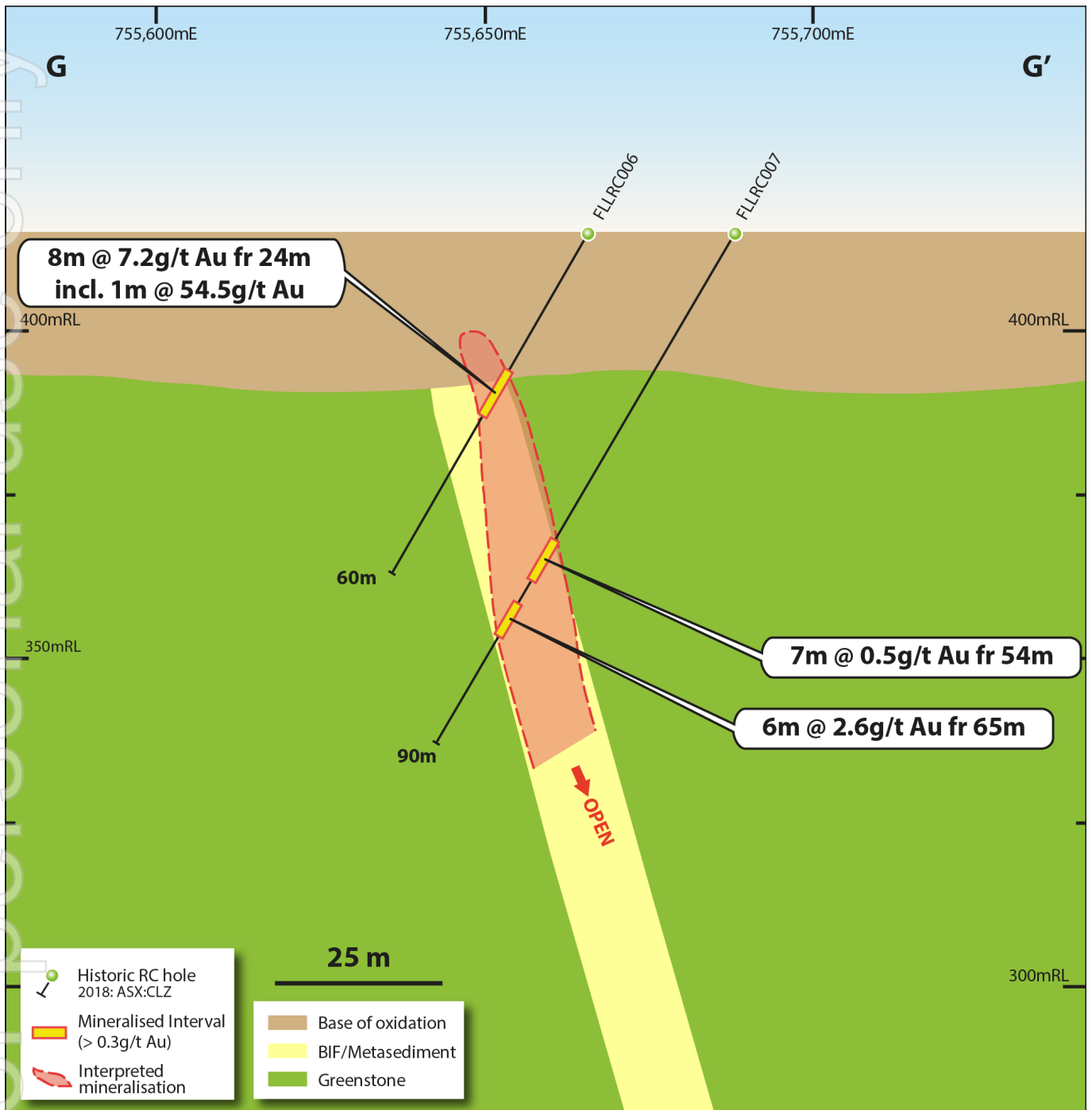
Figure 11. Cross section (G-G'), looking north ~8m along strike, showing Au mineralisation of historic drilling. Drilling intercept widths are down-hole widths and not true widths. Intercepts are based on a cut-off grade of 0.3g/t Au, allowing for internal dilution by two "waste" or sub-grade (<0.3g/t Au) samples.
