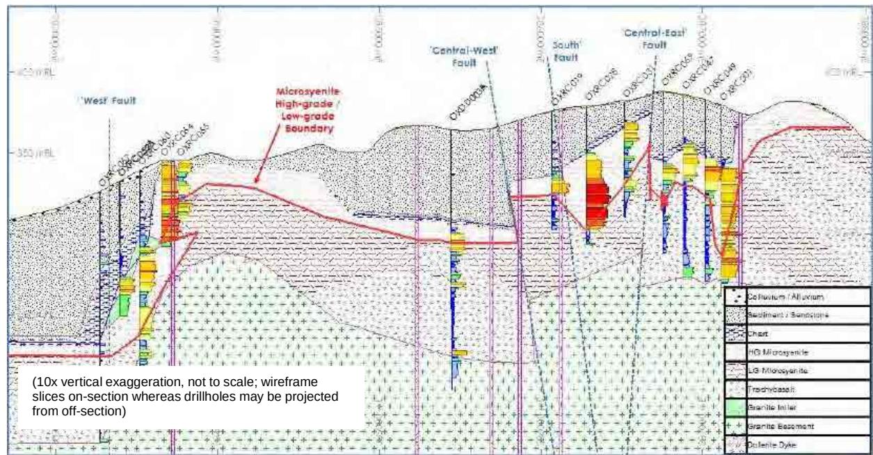
Figure 3-19: Example Cross Section at 6,768,600 mN showing Microsyenite High-Grade / Low-Grade Mineralisation Boundary
