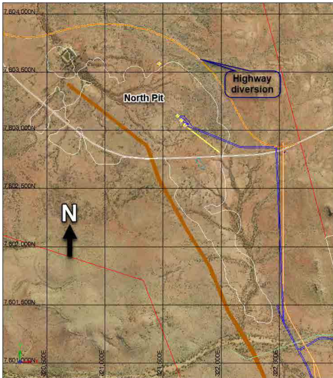
Figure 2-19: Proposed Pit and Waste Dump Layout for the Northern Zone from the 2018 DFS
