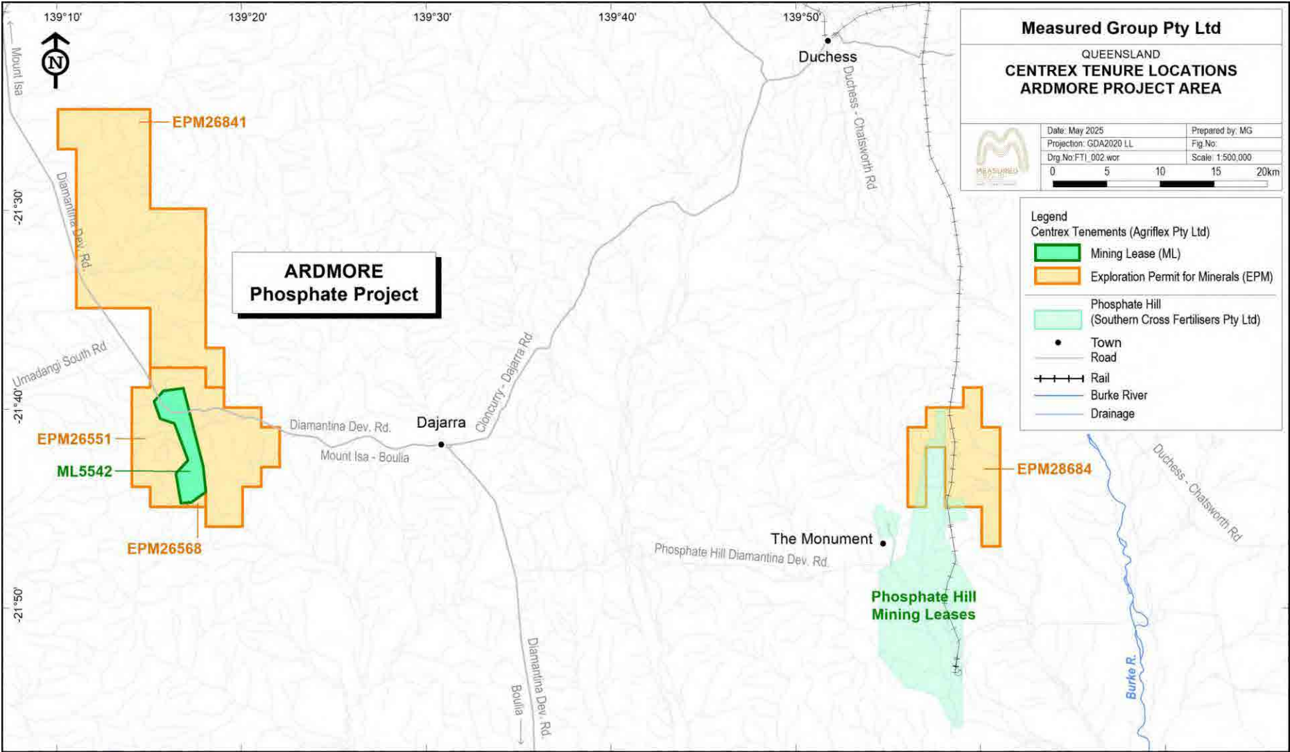
Figure 2-4: Location of Ardmore Phosphate Project Tenements
