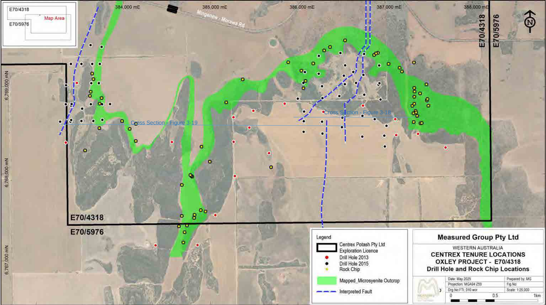
Figure 3-17: Plan of Oxley Exploration and Fault Interpretation with Cross Section Locations
