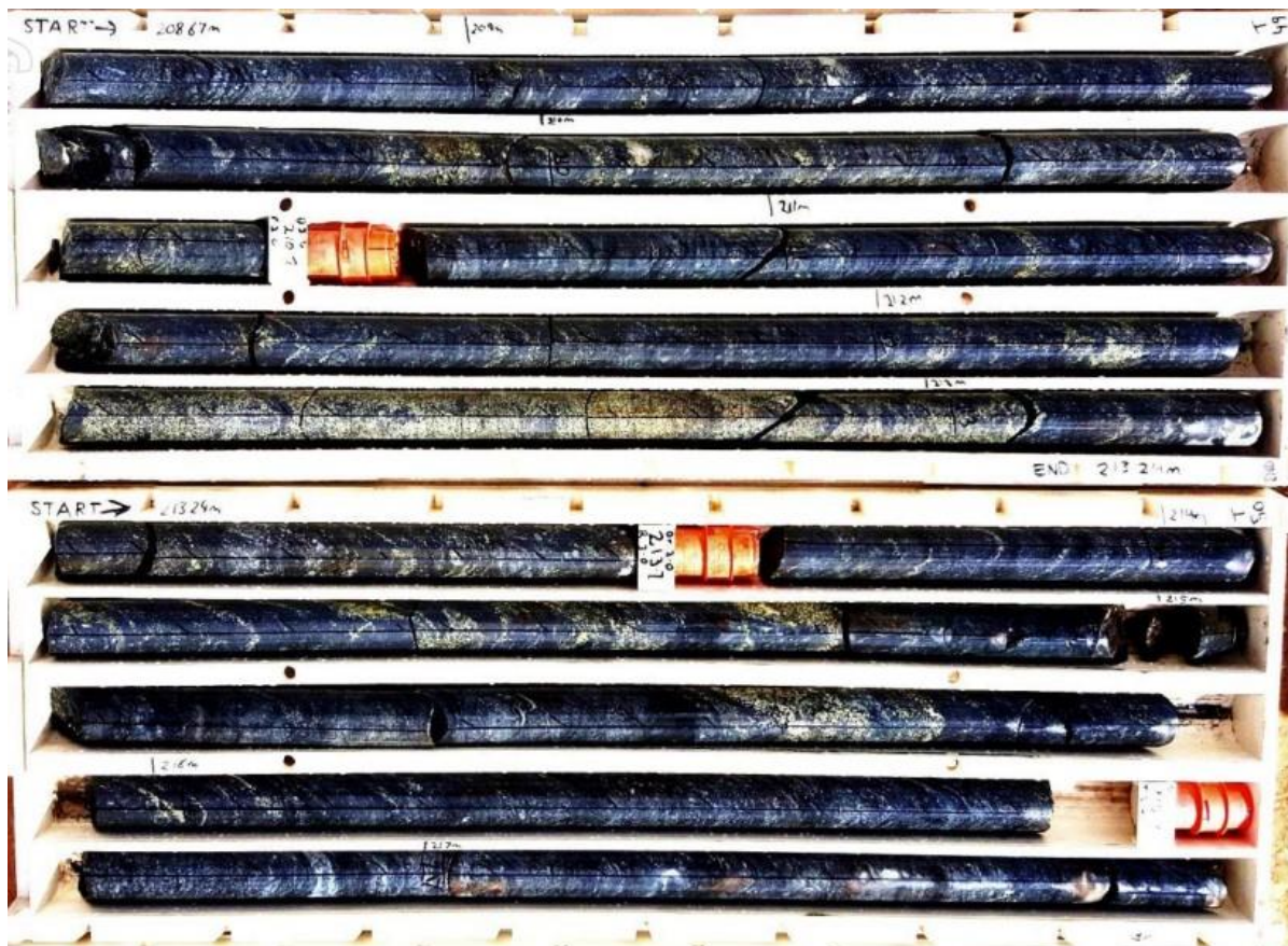
Hole 18CB054 intersection disseminated chalcopyrite-pyrite with accessory pyrrhotite in magnetite-chlorite quartz shear, 7m @ 1.97% Cu and 0.48 g/t Au from 208m downhole ( see assay table)
