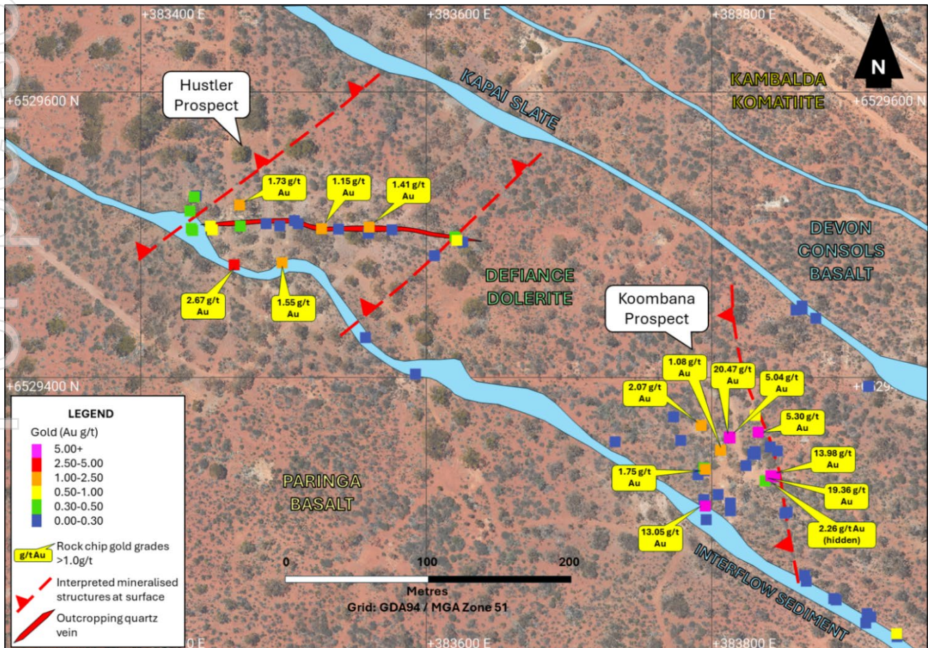
Figure 5: Plan view of the immediate Hustler and Koombana prospects showing surface sampling results and highlights (>1.0g/t Au).
