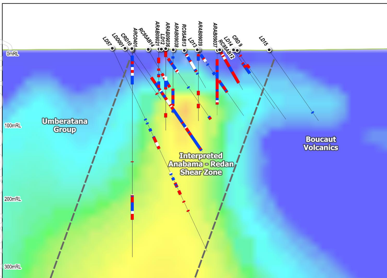
Figure 4: Orientation IP Survey Line F-F' with anomalous copper and gold drilling results 2 over chargeability inversion results and interpreted geology
