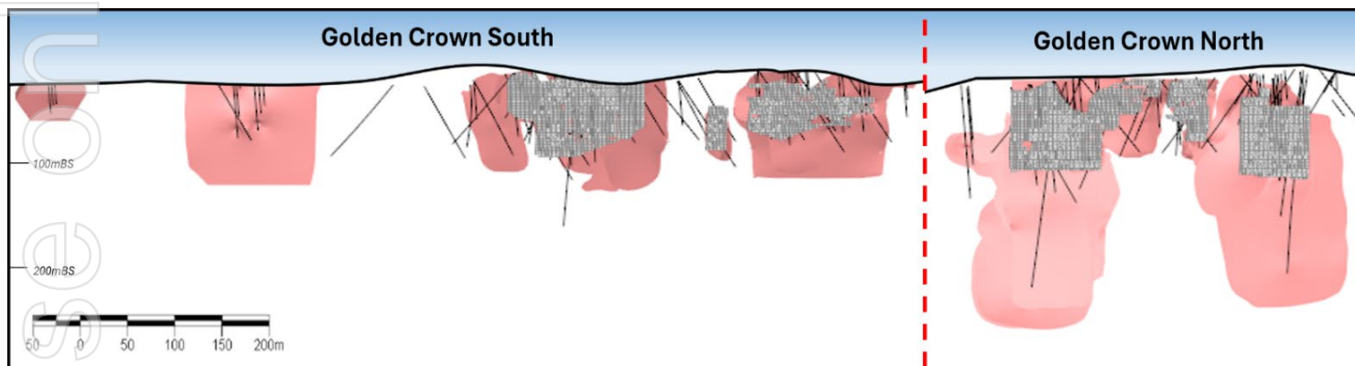
Figure 5: Golden Crown Exploration Target mineralisation envelopes (red fill) with 2021 MRE block model (grey) and drillhole traces (black) looking north-west. Dashed red line represents 500m of strike between Golden Crown South and North images for illustration purposes only.
