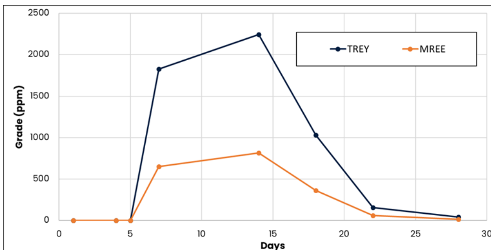
Figure 1. Solution concentration of rare earth elements in (ppm) over the 28-day test period.
