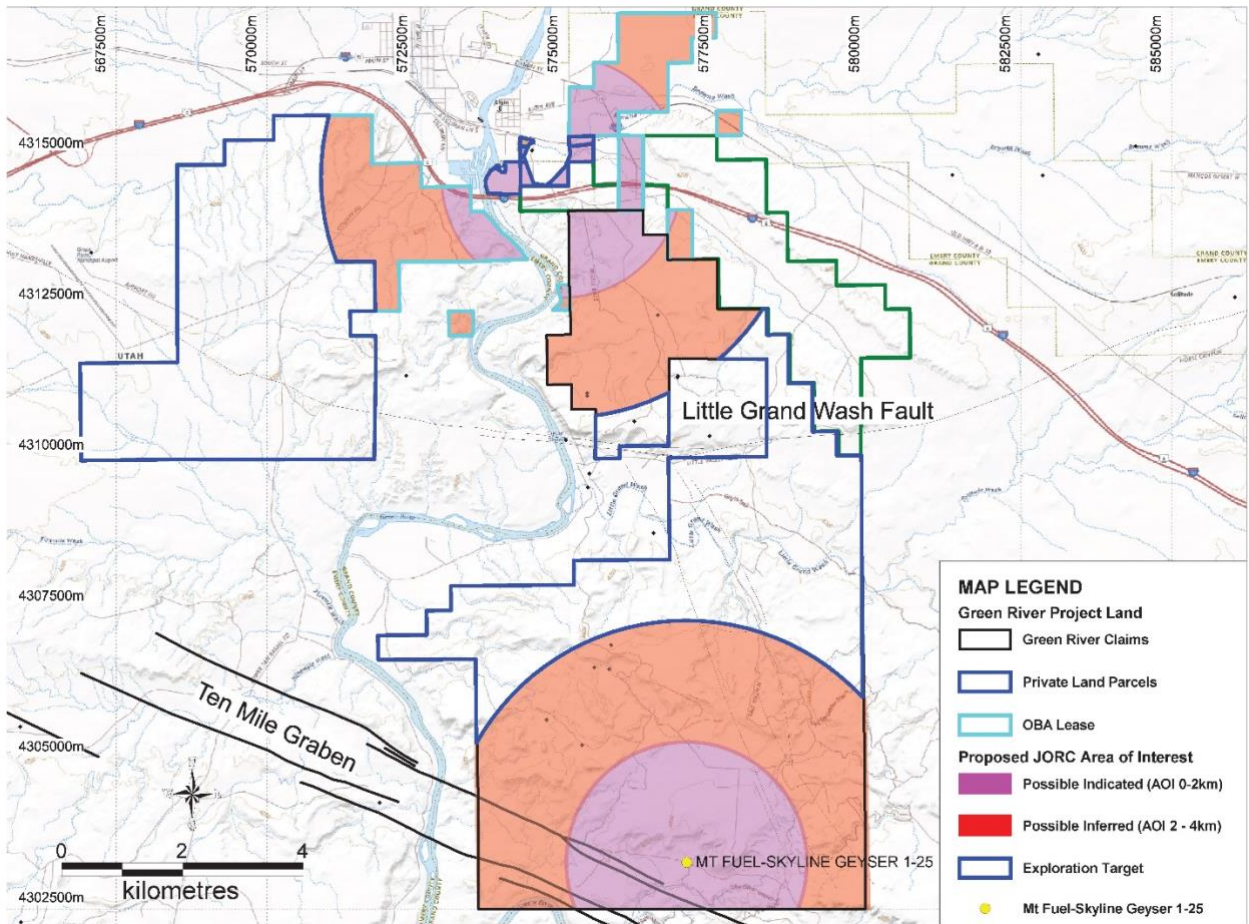
Figure 3: Proposed areas of interest on for the Green River Project after re-entering the Mt Fuel-Skyline Geysers 1-25 well.
