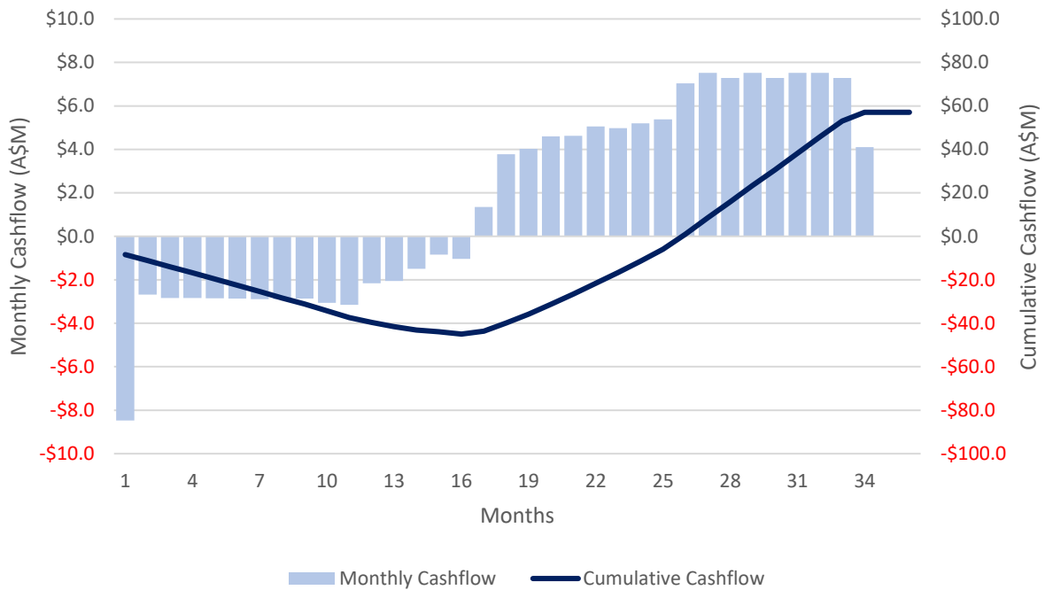
Figure 10: Monthly and Cumulative cashflow for the Mt Boppy cutback based on a gold price of A$5,000.
