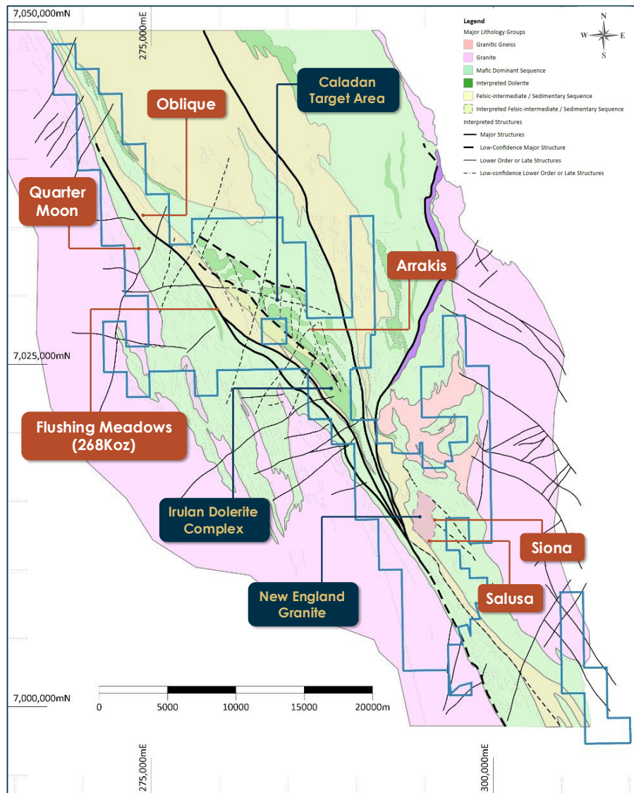
Figure 2: Simplified geology plan across the IWB Gold Project showing active prospects and exploration target areas, including the Siona and Arrakis Prospects.
