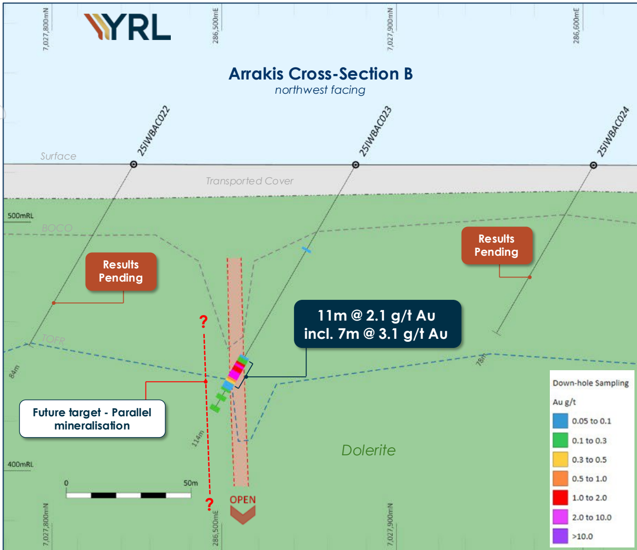
Figure 8: Cross-section showing all AC drilling results from 25IWBA023 , with a simple preliminary interpretation of geology. The section location is shown in Figure 6 . The section shows all drilling within +/- 50m of the section plane. The red line represents a potential future drill target, based on geological observation from intercepts 400m and 800m to the southeast. Please note that assay results from drilling adjacent to 25IWBA023 have not yet been received and are expected in the coming weeks.
