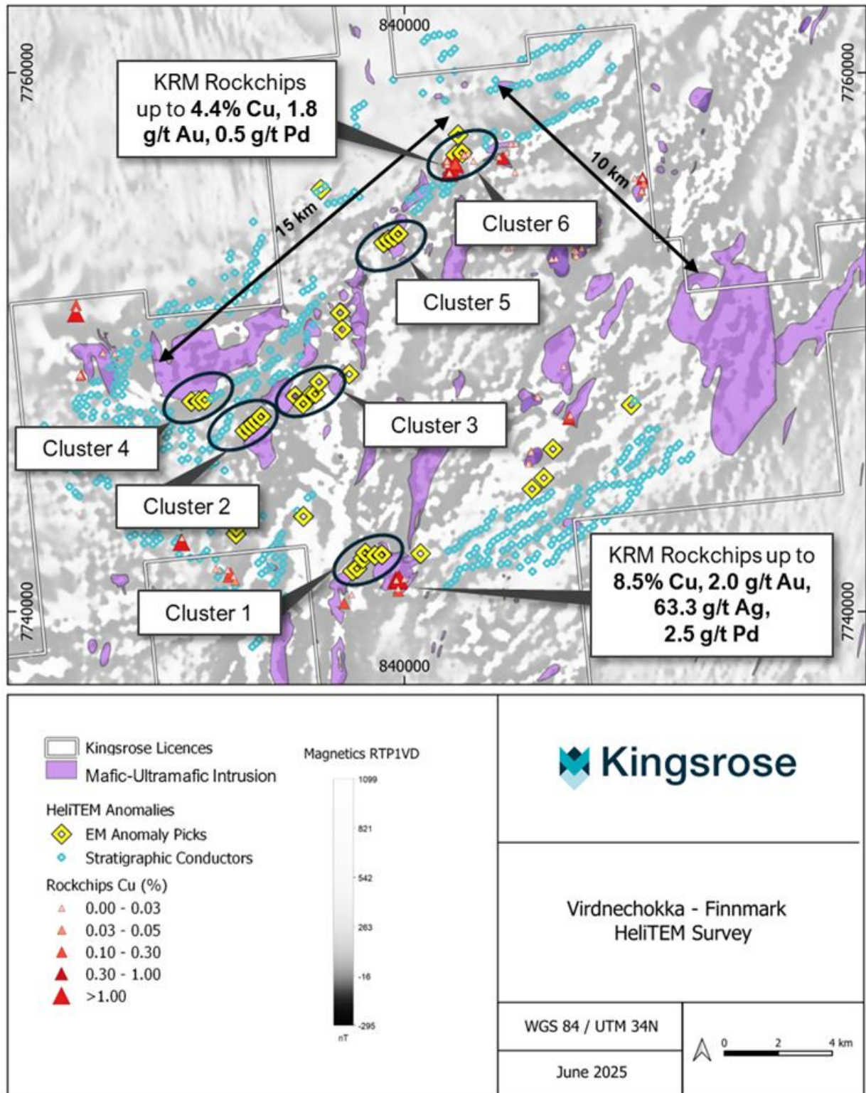
Figure 3: HeliTEM anomaly picks overlain on RTP1VD magnetic data and thematic copper rock chip results, Viridnechokka area
