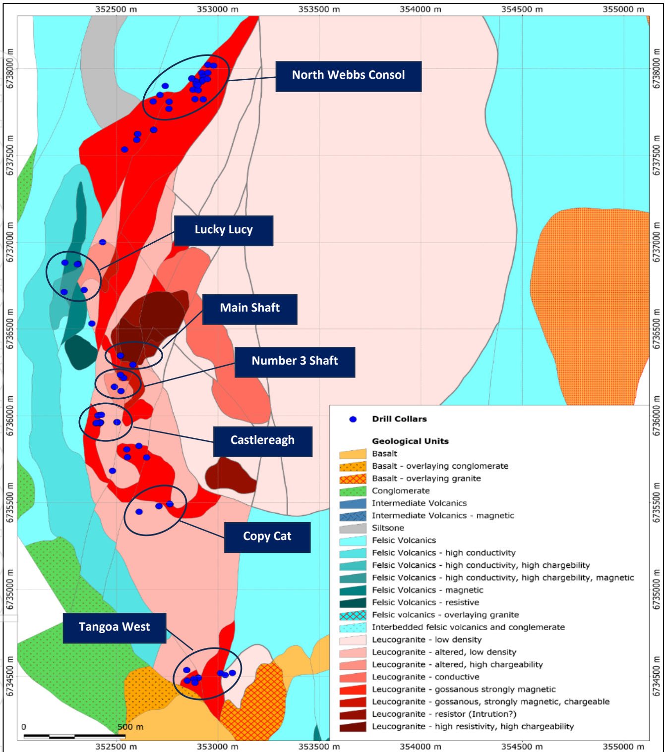
Figure 13. Webbs Consol project geology, mineralised lode locations and 97 drill collar positions
