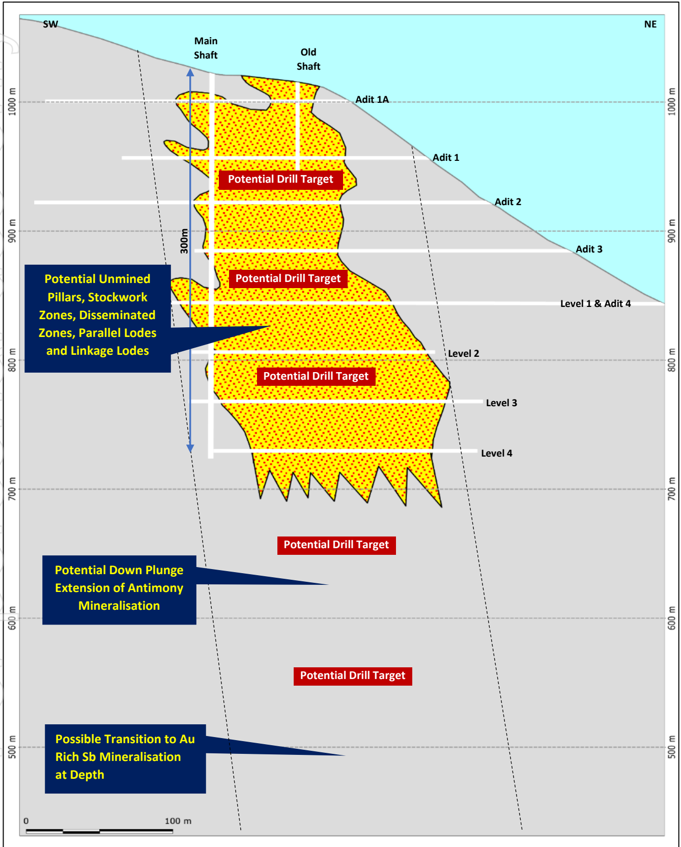
Figure 11. Magwood antimony mine longitudinal section - workings, stoped, potential unmined and down dip extensions of mineralisation
