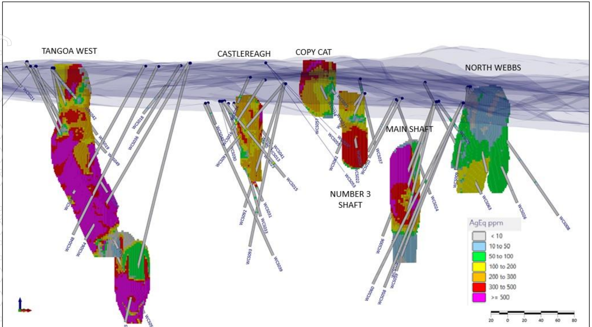
Figure 14. Long section of Webbs Consols mineralised pipes
