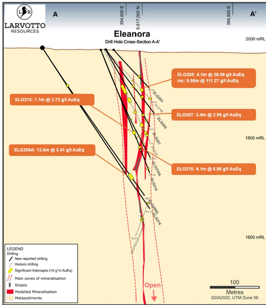
Figure 4 Eleanora-Garibaldi Cross-section A-A
