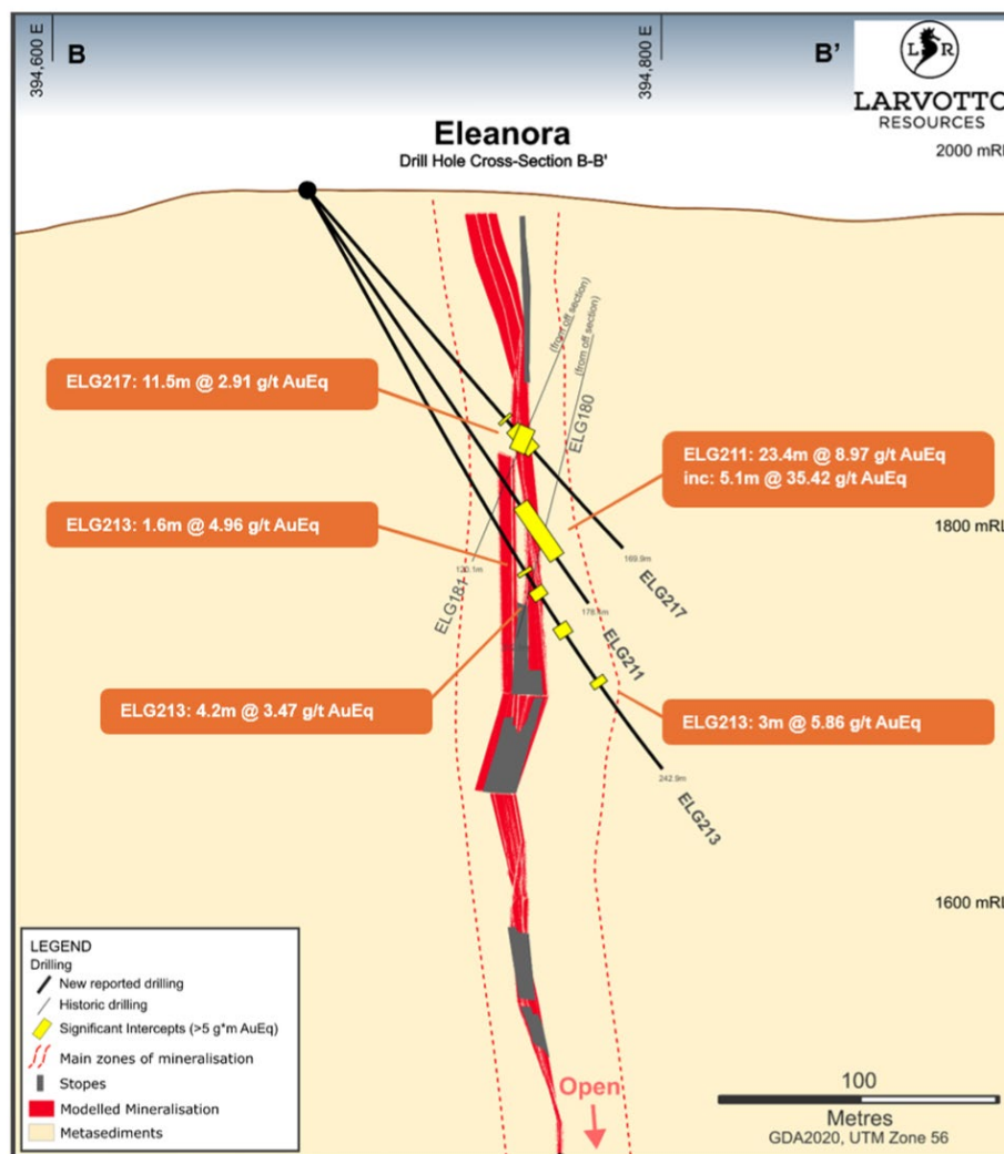
Figure 5 Eleanora-Garibaldi Cross-section B-B
