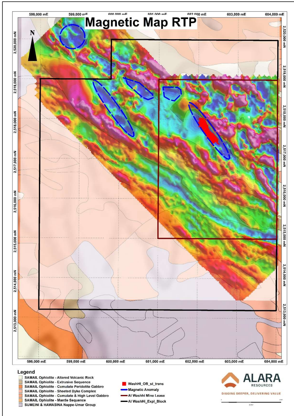
Figure 13: Geological Map overlain with potential RTP magnetic regional exploration targets in Al Wash-hi Majaza greenfield block
