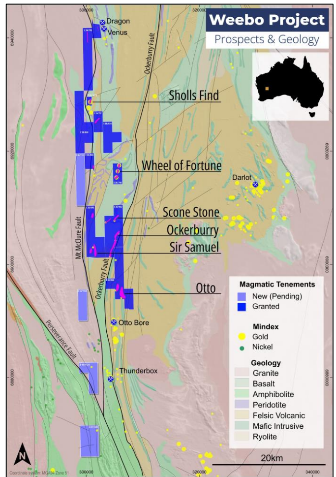
Figure 3: Weebo - Prospect locations on regional geology
