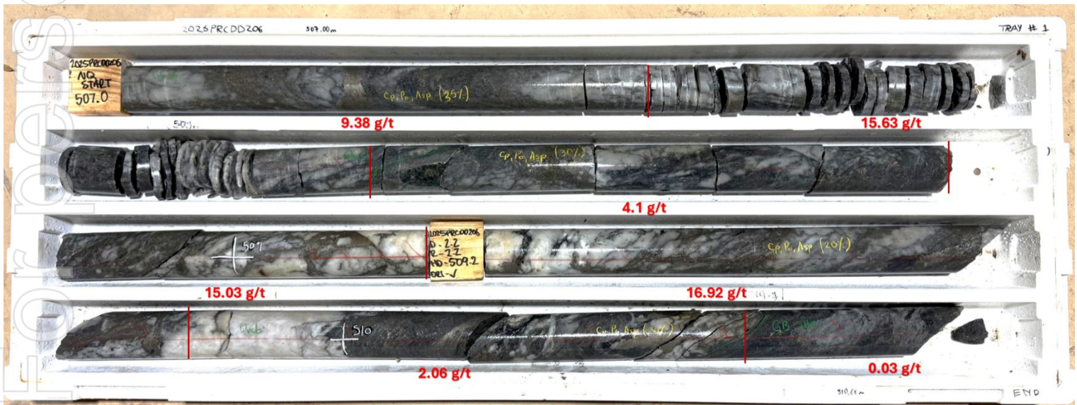
Figure 3 Core tray from hole 25PRCDD206, covering the interval from 507m to 510.9m. Intense, pervasive quartz-carbonate veins, with boudinage, folding, and curved veins, indicating ductile deformation and multiple fluid pulses with sulphides (pyrrhotite, arsenopyrite) with portions of grey colour mafic host rock.
