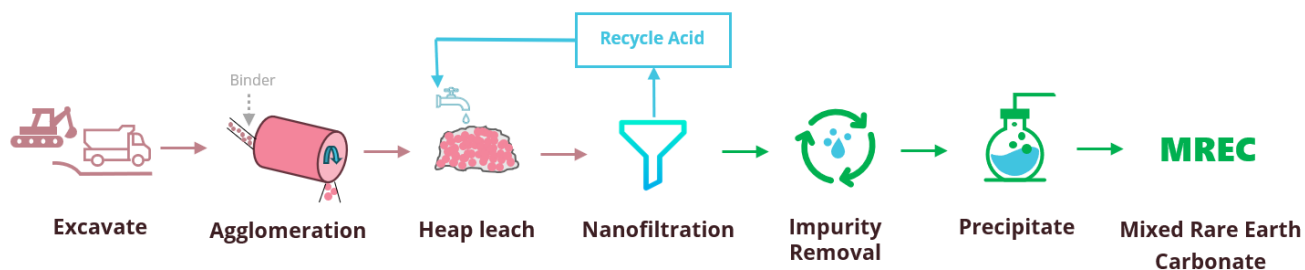
Figure 2: Indicative processing steps Heap Leach with Nanofiltration
