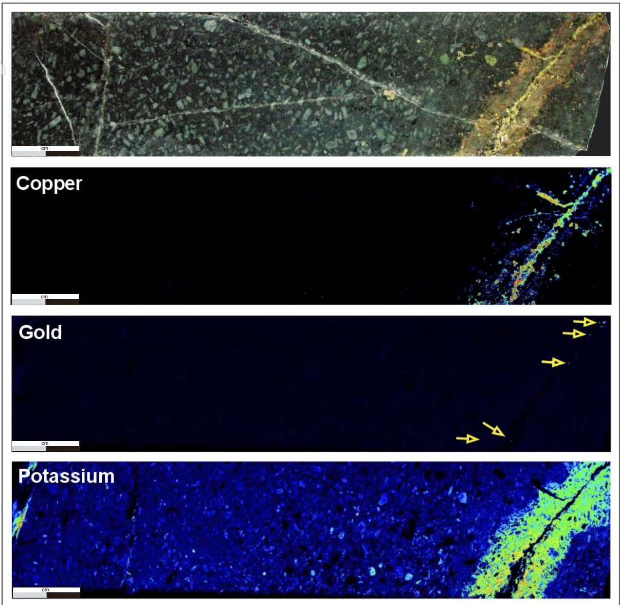
Figure 5: Micro XRF scans are being used to obtain detailed gold department information. Scans from SPRCD062 at 669m which returned a 43.3g/t Fire Assay. Screen Fire Assays are pending
