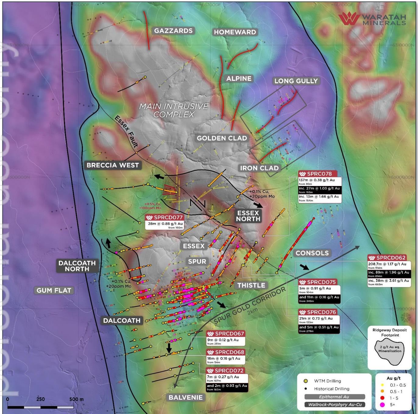
Figure 6: Spur Project, Main Intrusive Complex Targets, Spur Gold Corridor, and other epithermal and porphyry targets, drilling coverage, major surface geochemical trends over RTP magnetics. Ridgeway Deposit outline from Holliday et al 2000
