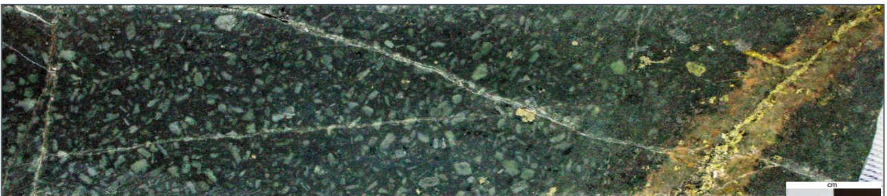
SPRCD062 - 669.7m – Veinlet chalcopyrite + quartz ± pyrite with strong k-feldspar vein halo, 43.3g/t Au
