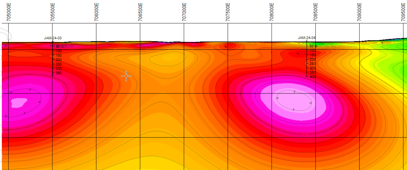
Figure 2. Section of the original 2D inversion model section for L7410300mN with drill holes Jam24-03 and -04 shown.
