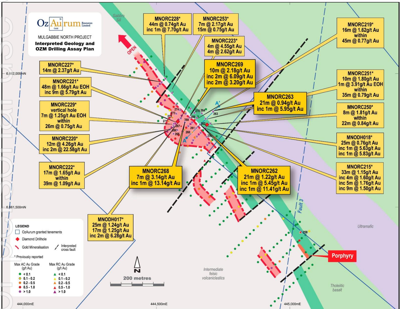
Figure 1: Cross Fault RC drill hole location plan.
