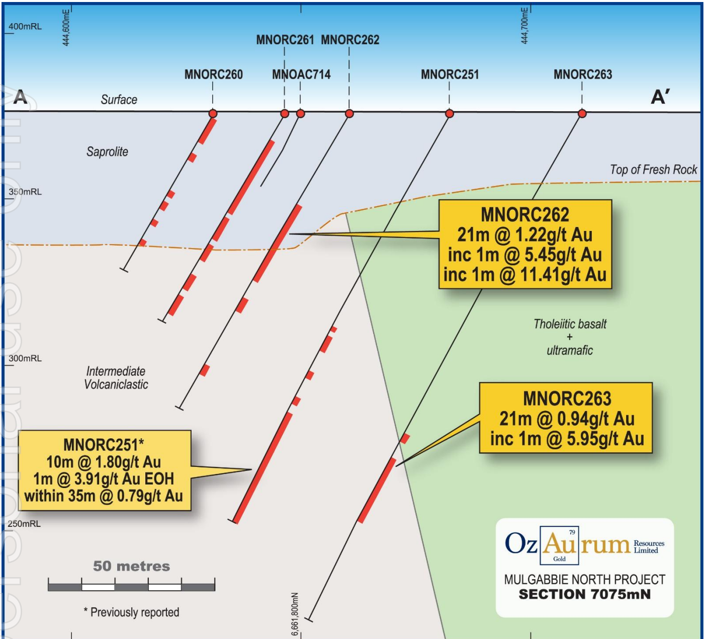
Figure 2: Cross Fault cross section 7075N
