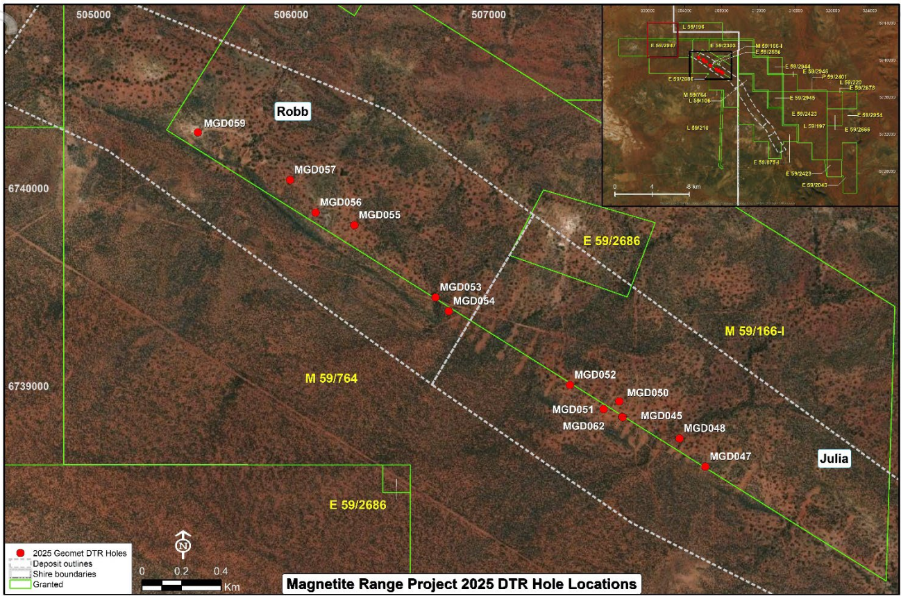
Figure 2: Drillhole location plan illustrating diamond holes over which 2025 DTR composite samples were collected.
