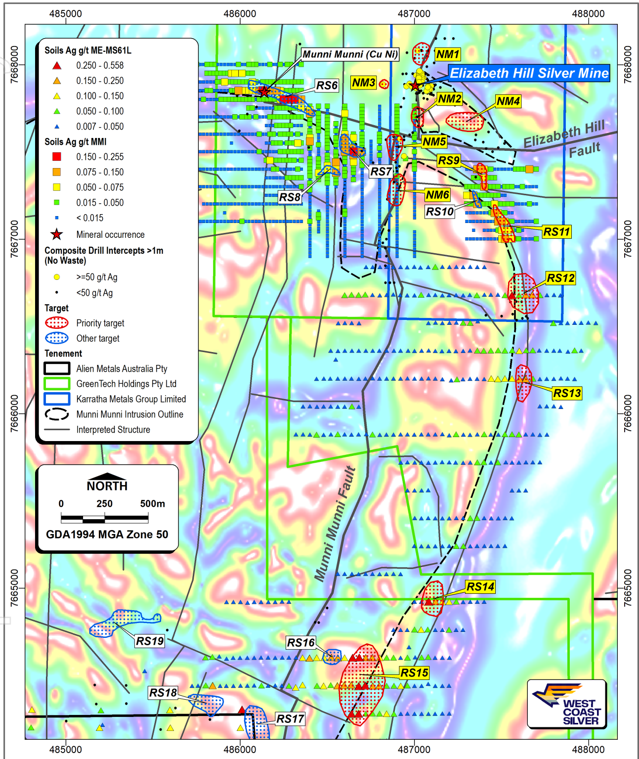
Figure 8.- Further top.76 targets along the east side of the Munni Munni intrusion. (Overlaid on RTP Band Pass Filter Tilt Magnetic Image)
