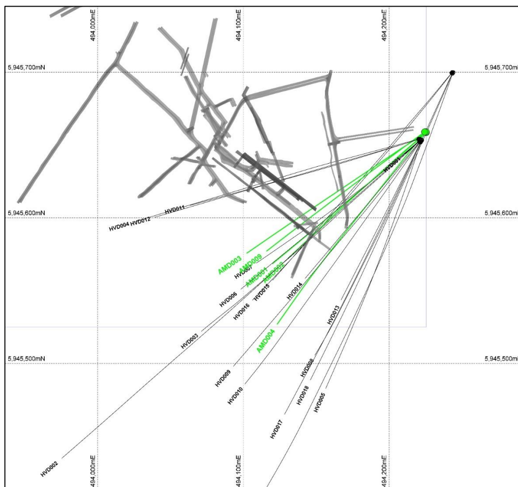
Figure 5. Plan view showing locations of recent Advance Metals holes AMD001-004 and AMD009 (green) in reference to previous drill holes (black) and historic workings (grey) at the Happy Valley Prospect at Myrtleford.
