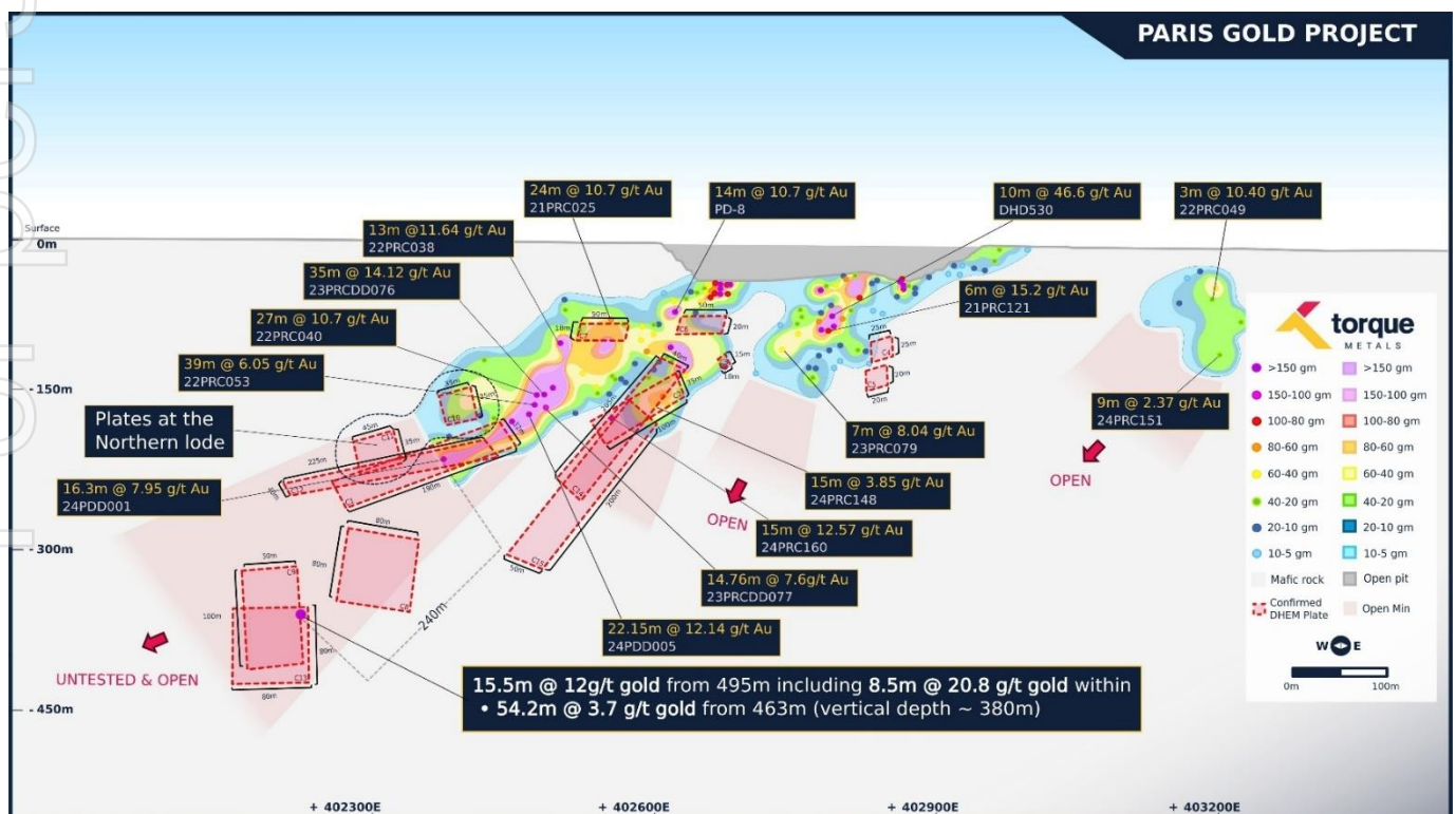
Figure 1 EM conductor plates modelled from DHEM surveys targeting extensions of gold-associated sulphide minerals.
